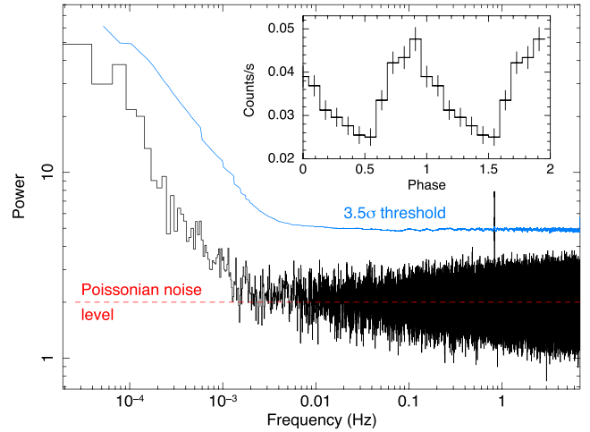
Figure 1. Fourier power spectrum from the 2000 December–2013 February pn data (0.5–10 keV; average of 36 Fourier transforms; \Delta t \simeq 73 ms, 262 144 frequencies). The blue line corresponds to the 3.5\sigma confidence level threshold for potential signals and was computed taking into account the number of trials, equal to the number of frequency bins of the spectrum. The prominent peak above the threshold corresponds to the 1.2-s signal. The inset shows the light curve of the data set 0650560301 (where the signal was discovered) folded to its best period.
