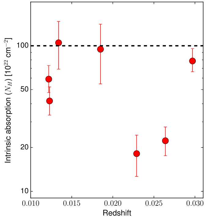
Figure 1. Intrinsic absorption N_{\text{H},z} computed assuming \theta = 90^\circ as a function of redshift for the seven sources in our sample. The horizontal dashed line marks the Compton-thick regime (i.e., N_{\text{H},z} \geq 10^{24} \text{ cm}^{-2} ).
