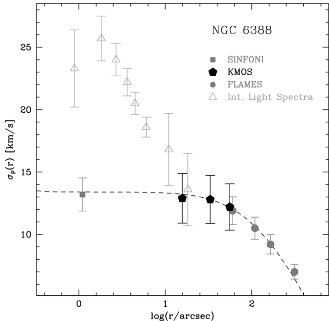
Figure 9. Line-of-sight velocity dispersion profile of NGC 6388 computed from the radial velocities of individual stars, as measured with KMOS (black pentagons, this paper), SINFONI, and FLAMES (dark gray squares and circles, respectively; from L13). The dashed line correspond to the self-consistent King model plotted in Figure 13 of L13. The velocity dispersion profile obtained from integrated-light spectra (Lützgendorf et al. 2011) is also shown for comparison (light gray empty triangles).
