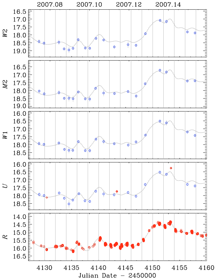
Fig. 2. UVOT light curves of AO 0235+164 compared to the ground-based U data from the NOT (red diamonds) and to the R -band data ( bottom panel ). All data have been corrected for the ELISA contribution. The cubic spline interpolation through the 1-day binned R -band light curve is shown in each panel, properly rescaled (see text).
