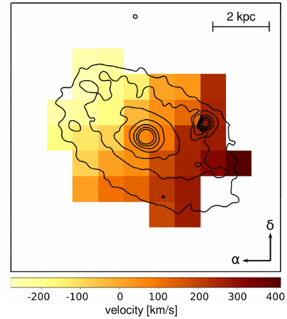
Figure 1. [C\text{II}] line-of-sight velocity map of NGC 7049 based on Werner et al. (2014). Values are relative to the systemic velocity of the galaxy. The velocity distribution of the [C\text{II}] emitting gas indicates the presence of a disc, rotating with a velocity of v_{\text{rot}} \sim 200\ \text{km s}^{-1} .
