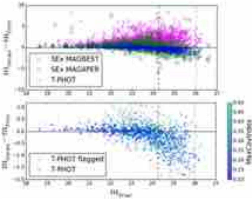
Fig. 16. Top : measured magnitude differences ( m_{\text{meas}} - m_{\text{true}} ) versus “true” input magnitudes m_{\text{true}} , for two simulated images populated with extended sources (HRI has FWHM = 0.2'' and HST H -band-like fluxes, LRI has FWHM = 1.66'' and IRACch1-like fluxes), using three different methods: SEXTRACTOR dual-mode aperture, SEXTRACTOR dual-mode “best”, and T-PHOT. Vertical lines show the 5\sigma (dashed) and 1\sigma (dotted) limits of the simulated LRI. Bottom : magnification of the top panel , showing only T-PHOT results, colour-coded as a function of the covariance index. See text for more details.
