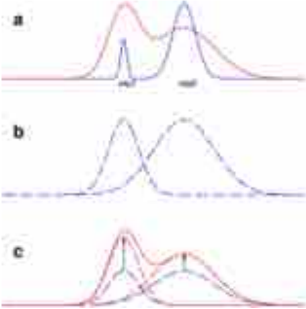
Fig. 1. Schematic representation of the PSF-matched algorithm implemented in T-PHOT. Top : two objects are clearly detected and separated in the high-resolution detection image (blue line). The same two objects are blended in the low-resolution measurement image and have different colours (red line). Middle : the two objects are isolated in the detection image and are individually smoothed to the PSF of the measurement image, to obtain normalized model templates. Bottom : the intensity of each object is scaled to match the global profile of the measurement image. The scaling factors are found with a global \chi^2 minimization over the object areas. Image from De Santis et al. (2007).
