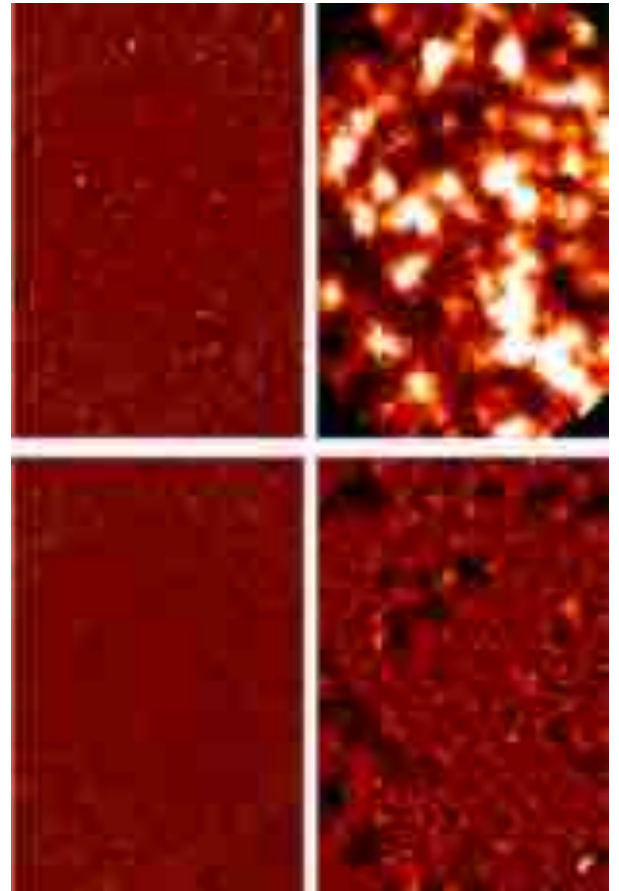
Fig. 19. Results from a test run using T-PHOT with unresolved priors on FIR/sub-mm real dataset. Upper row, left to right : SCUBA-2 450\ \mu\text{m} ( FWHM = 7.5'' ) and Herschel 500\ \mu\text{m} ( FWHM = 36'' ) images of the COSMOS-CANDELS fields. Lower row, left to right : residuals for the two fields, obtained with T-PHOT runs using a list of 24 + 850\ \mu\text{m} priors. See text for details.
