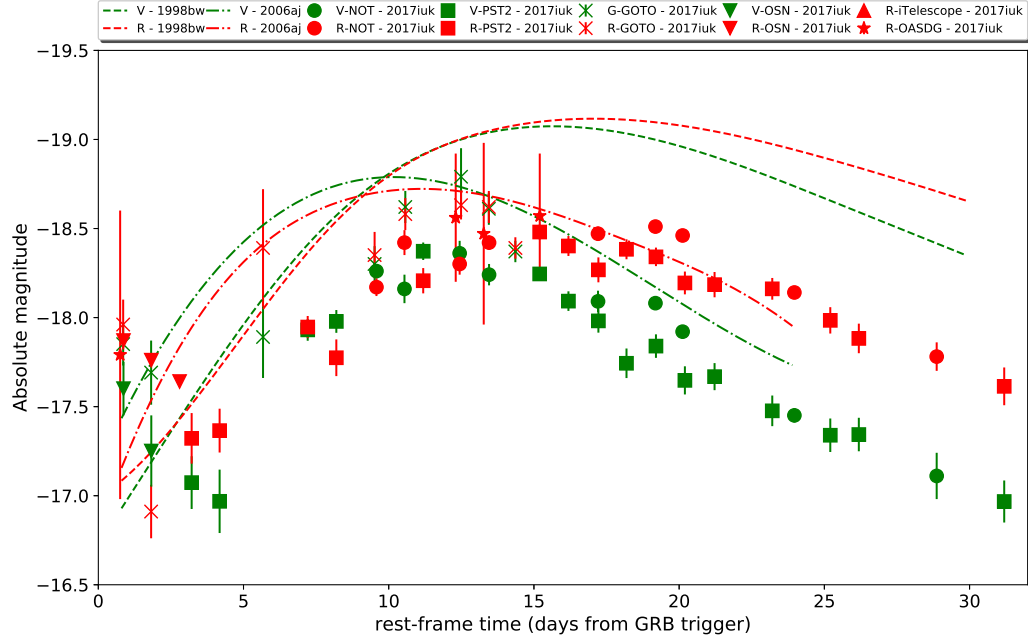
Figure 8. SN 2017iuk vs. SN 1998bw and SN 2006aj. Evolution of the V (green) and R_C (red) absolute magnitudes for SN 2017iuk as observed from the NOT, the OSN, the RBT/PST2, the GOTO and smaller telescopes (iTelescope, OASDG). The evolution in the first 30 days of SN 1998bw (dashed curves) and SN 2006aj (dot-dashed curves) are also shown, considering a common rest-frame time interval. Error bars represent 1 s.d..
