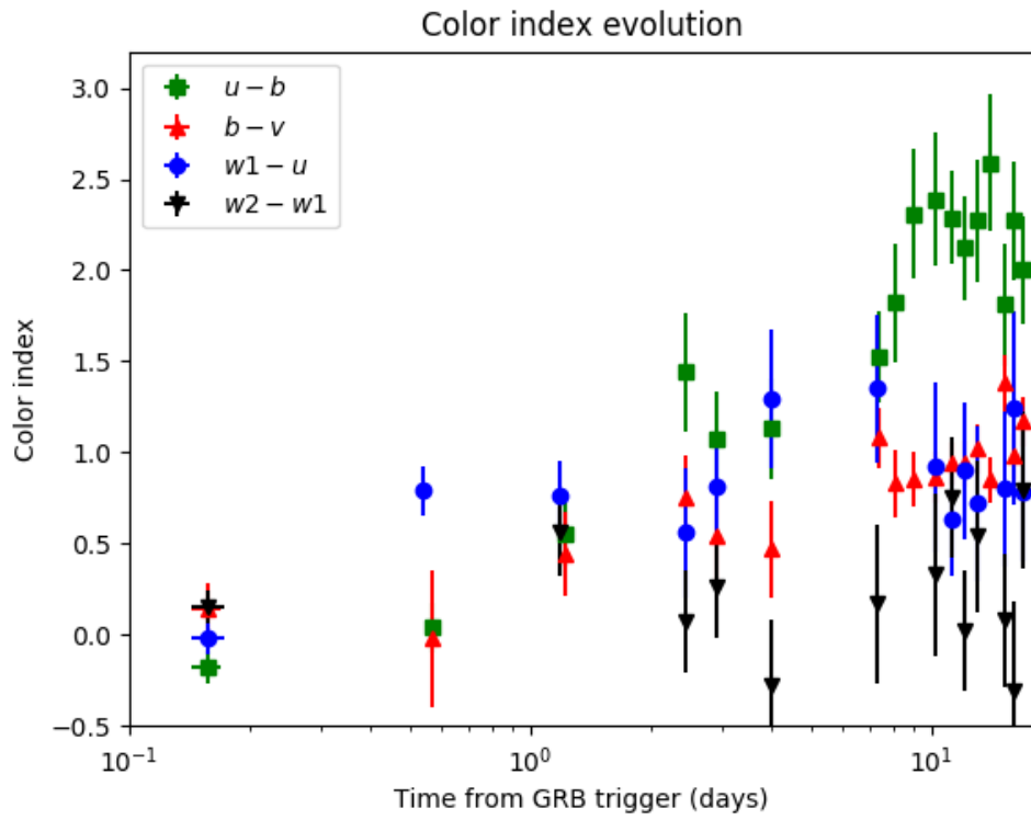
Figure 5. The early colour index evolution. The u-b , b-v , uvw1-u and uvw2-uvw1 colour index evolution, computed from UVOT data in the first 18 days after the GRB trigger. Error bars represent 1 s.d..
