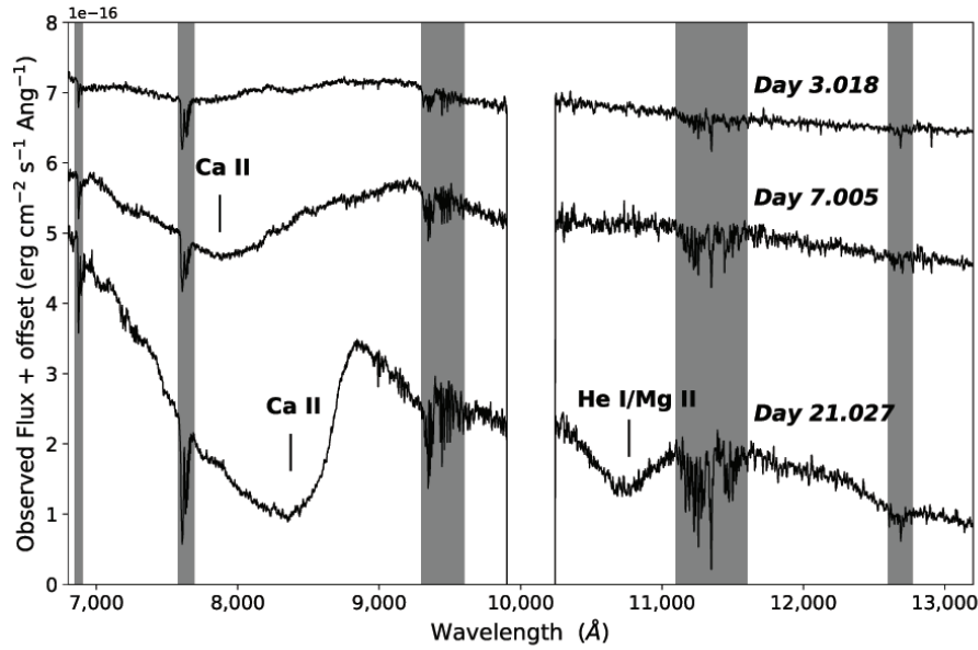
Figure 10. Spectroscopic evolution of SN 2017iuk in the near-IR wavelength range. Gray regions indicate telluric features in the spectra. The possible He I \lambda 10830 / Mg II \lambda 10914 feature is visible in the day 21 spectrum, while the Ca II triplet shows a P-Cygni profile at bluer wavelengths.
