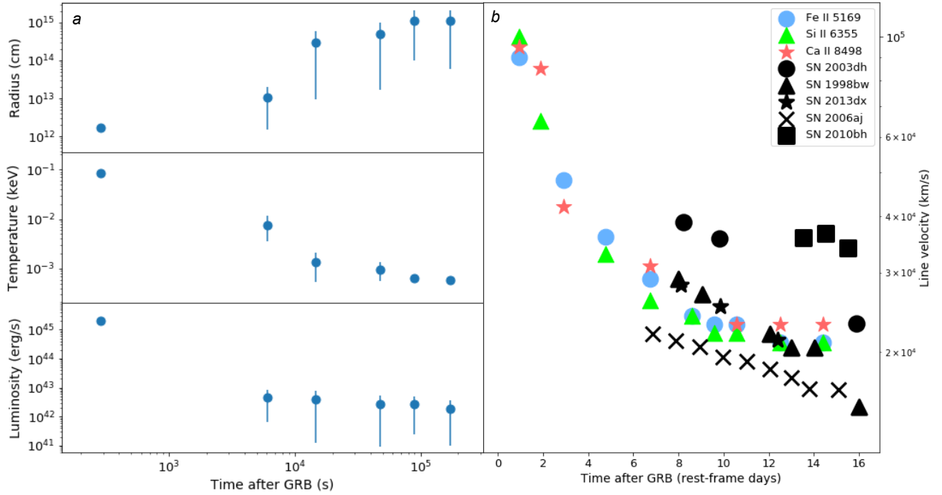
Figure 3. (a) Temporal evolution of the blackbody model parameters: from the top: radius, temperature and luminosity of the blackbody as a function of time since the GRB detection. (b) The velocity variation estimated from the absorption line of FeII \lambda 5169 , SiII \lambda 6355 and CaII \lambda 8498 in the SN 2017iuk spectra up to Day 16. For comparison we show the velocity estimated from the absorption of SiII \lambda 6355 for the following GRB-SNe: GRB 980425/SN 1998bw 1 , GRB 030329/SN 2003dh 2 , GRB 060218/SN 2006aj 16 , GRB 100316D/SN 2010dh 15 and GRB 130427A/SN 2013dx 17 .
