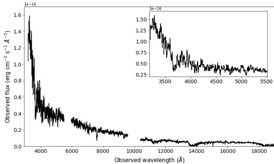
Figure 9. The spectrum of GRB 171205A/SN 2017iuk obtained 1.5 hours after the GRB detection. This spectrum has been obtained with VLT/X-shooter in the range 3200 – 19000 Å. The inset shows the UVB arm (3200 – 5500 Å), where the emission excess at wavelengths \leq 4000 Å and a possible absorption feature at \sim 3700 Å are shown.
