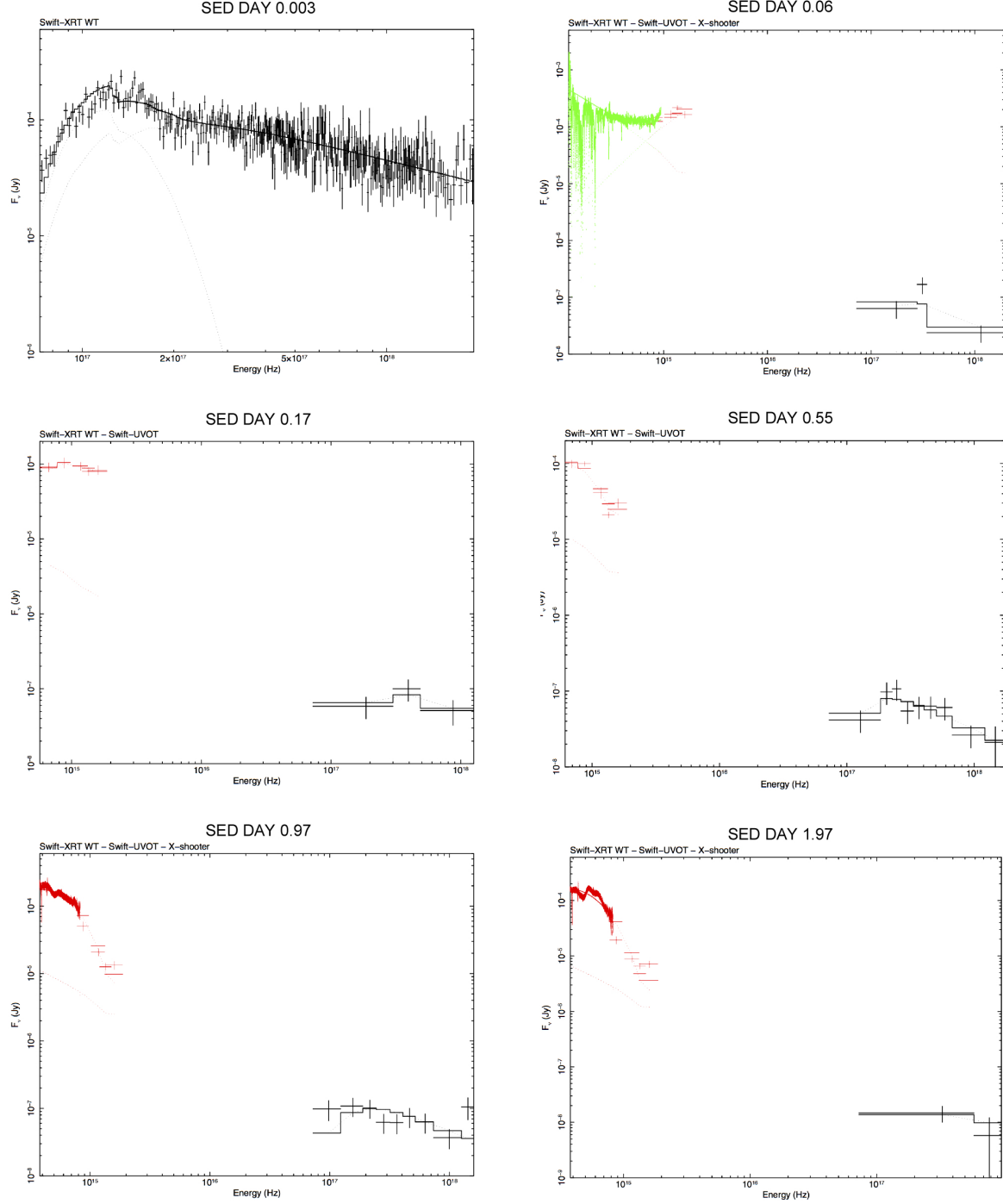
Figure 6. The modelling of the spectral energy distributions. SEDs for the epochs at ( top ) T_{SED1} = 0.003 days and T_{SED2} = 0.06 days, ( middle ) T_{SED3} = 0.17 days and T_{SED4} = 0.55 days, ( bottom ) T_{SED5} = 0.97 days and T_{SED6} = 1.97 days. All data sets use photometric data points obtained with Swift UVOT for the low-energy part of the spectrum. Error bars represent 1 s.d. The SED is complemented with VLT/X-shooter and GTC/OSIRIS spectra for the epochs at days 0.06, 0.97 and 1.97, respectively, while for the X-ray energy range we built specific Swift XRT spectra. An additional spectrum is shown in the top-left panel together with the best-fit results obtained for the Swift windowed timing mode spectrum computed at 0.003 days using a blackbody + power-law spectral model.
