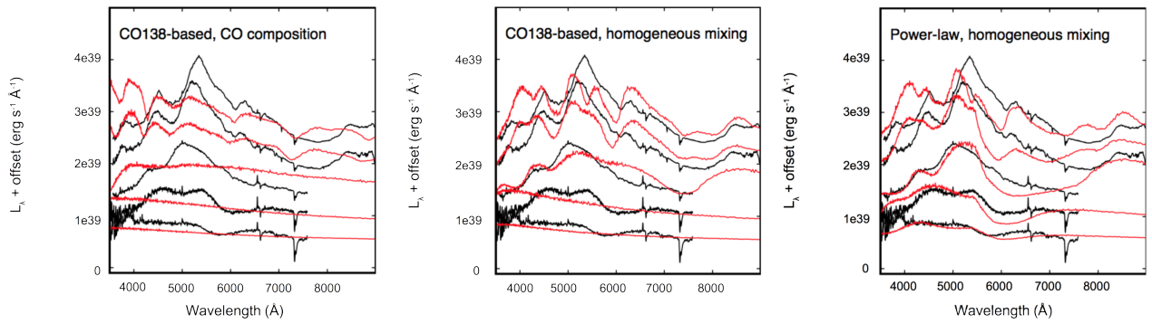
Figure 11. The observed spectral sequence of SN 2017iuk from Day 0.947 to Day 14.995 (red curves) as compared with spectral synthesis simulation (black curves) in the case of a C+O core abundance ( left panel ), in the case of a homogeneous mixing of the explosive elements 20 ( middle panel ) and in the case of a homogeneously-mixed power-law distribution ( right panel ). The differences with the results using the model considered in this work (see Fig. 2) are clearly evident.
