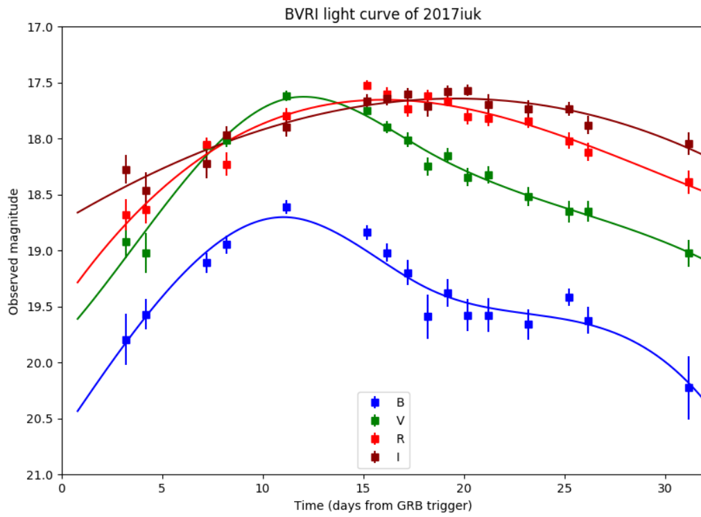
Figure 7. SN 2017iuk light curve evolution. BVR_{CLC} magnitude evolution of SN 2017iuk as observed with the RBT/PST2 telescope. Coloured curves represent the interpolation functions used for estimating the peak brightness. Error bars represent 1 s.d.
