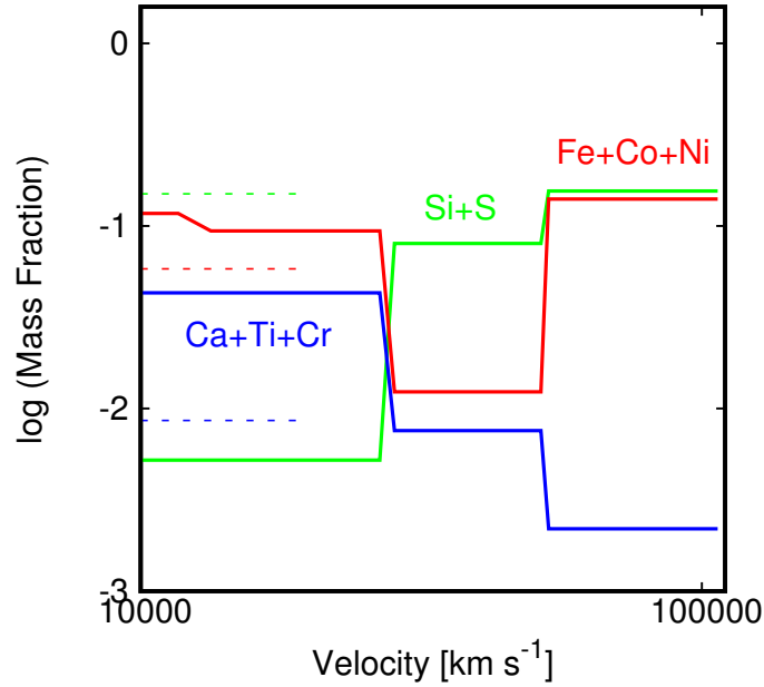
Figure 4. The abundance composition structure of the SN 2017iuk ejecta that is used in our spectral synthesis model. Dashed lines represent the homogeneous mixing levels of the explosive elements. At very high velocity we observe an increase in the abundance of Fe/Ni, which is expected when the GRB jet injects metal-rich blobs over a time-scale longer than the typical shock/jet breakout.
