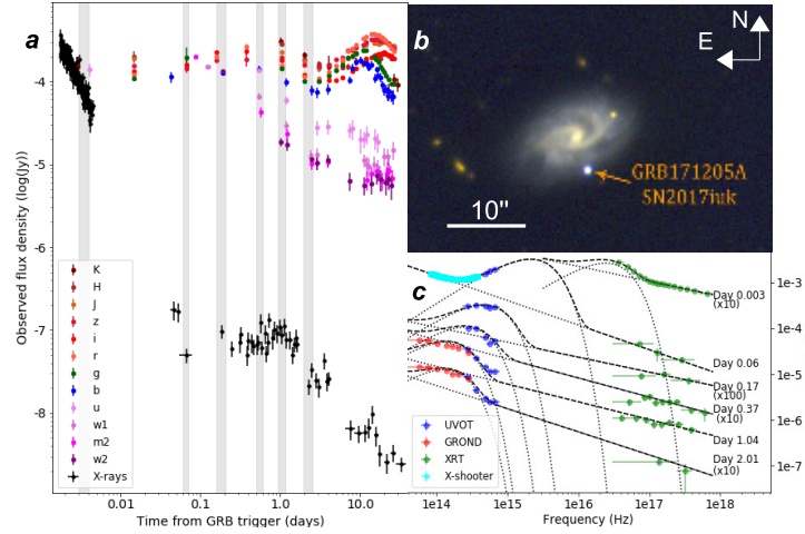
Figure 1. (a) Multi-wavelength light curve of the optical transient following GRB 171205A. During the first three days the optical, UV and NIR emission is dominated by a spectrally evolving bump. Beyond day three, a classical Type Ic supernova component emerges, SN 2017iuk. Grey regions correspond to the epochs of our multi-frequency SED analysis. (b) True-colour image of GRB 171205A/SN 2017iuk and its spiral host galaxy obtained with OSIRIS at the 10.4m GTC. (c) The best-fit results using one or two blackbodies plus a power-law spectral model for the six spectral energy distributions, obtained with Swift for UV and X-rays and ground telescopes (GROND and X-shooter), that are marked in panel (A).
