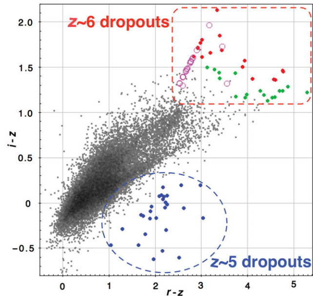
Figure 4. i-z versus r-z diagram for the LBC sources in J1030 field (small gray dots; \approx 30\,000 objects). LBC primary and secondary i -dropouts are shown as red- and green-filled circles, respectively. Magenta dots are even fainter i -dropouts ( 25.2 < z_{AB} < 25.5 ). All the i -dropout highlighted in the upper right part of the plot are undetected in the deep r -band ( r \sim 27.5 ) LBT image. The LBC z \sim 5 galaxy candidates are shown as blue dots.
