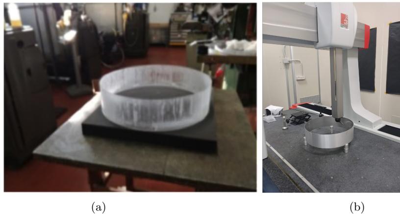
Figure 2: (a) One of the three single reflection shells obtained by cutting the double reflection configuration shells. (b) An aluminium shell under measurement with coordinate measurement machine.
