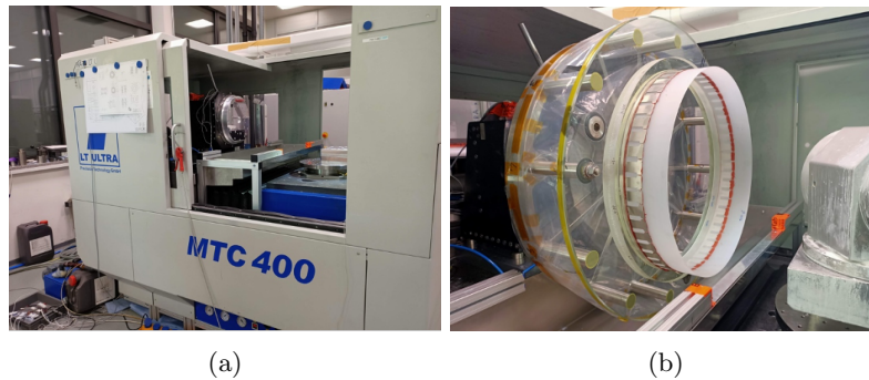
Figure 6: (a) Diamond turning lathe installed at LT-Ultra. (b) The shell in the S2 installed on board of the lathe. Plastic covers limit the liquid dispersion.
