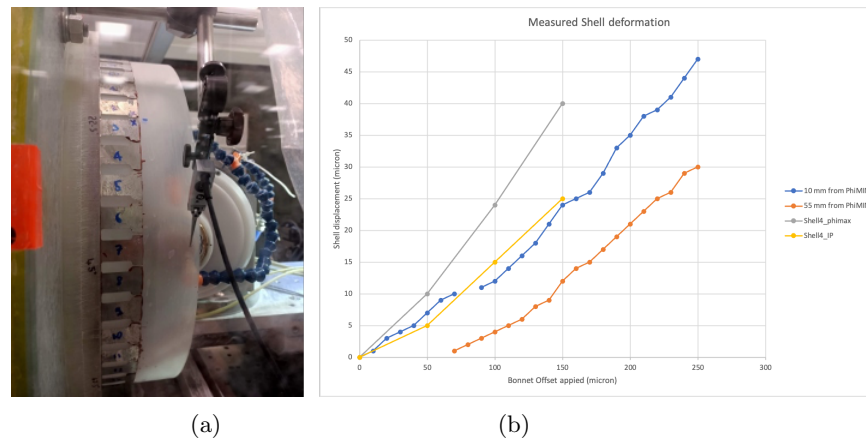
Figure 7: (a) Shell deflection measurement set-up. (b) Measured deformation on the back surface of the shell under machining in two different accessible positions, near the edge and near the flexures. Data are compared with the ones acquired on previous shell#4.
