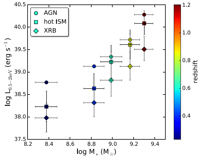
Figure 6. Nuclear X-ray luminosity (circles), hot ISM luminosity (squares) and XRB luminosity (diamonds) in the (0.5–2 keV) band vs. average stellar mass of each stacked redshift bin.
