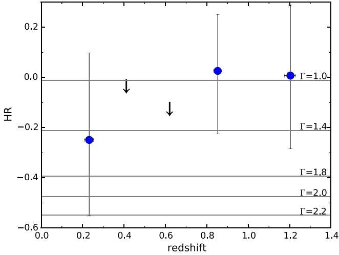
Figure 7. Hardness ratio vs. redshift for the five complete redshift bins. The lines indicate the HR from a population of XRBs with \Gamma = 1, 1.4, 1.8, 2, 2.2 (from top to bottom) and Galactic N_{\text{H}} .
