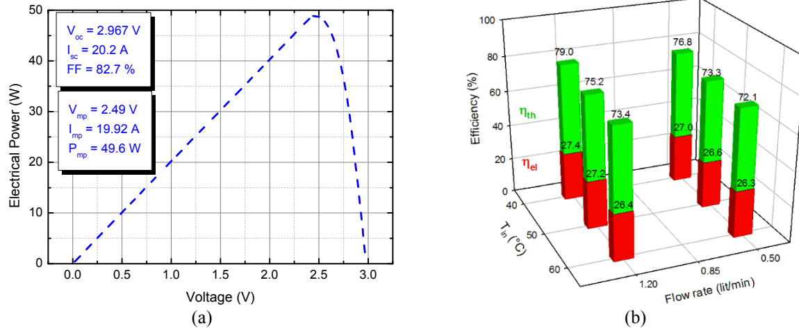
FIGURE 4. (a) PV curve obtained under a DNI of 900 \text{ W/m}^2 with a flow rate of 1.2 liters/min and inlet temperature of 40^\circ\text{C} . (b) Electrical (red), Thermal (green) and Total CHP efficiencies as a function of T_{in} and \dot{V} ; for each bar we indicate the values of electrical and total efficiencies.
