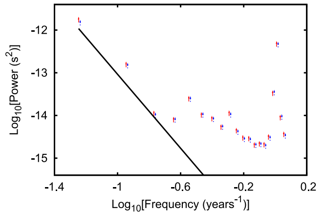
Figure 9. (Top) 95 per cent upper limits from an unparameterized power spectrum analysis for a correlated GWB (red points), and uncorrelated common red noise process (blue points) for the six pulsar data set described in Section 4 obtained while varying the intrinsic noise parameters for each pulsar. The upper limit obtained from a power-law analysis of the GWB at a spectral index of 13/3 of 3 \times 10^{-15} is overplotted as a straight line. Frequencies were included from 1/T up to 20/T , with T = 17.66 yr. Beyond these frequencies, the data provides increasingly poorer constraints on a steep red noise process, and so we do not consider higher frequency terms in our model. Both the correlated and uncorrelated power spectrum are completely consistent with one another at all frequencies. The difference in the log evidence between the correlated and uncorrelated models was 0.2 \pm 0.3 , indicating no support for the presence of a correlated signal in the data set.
