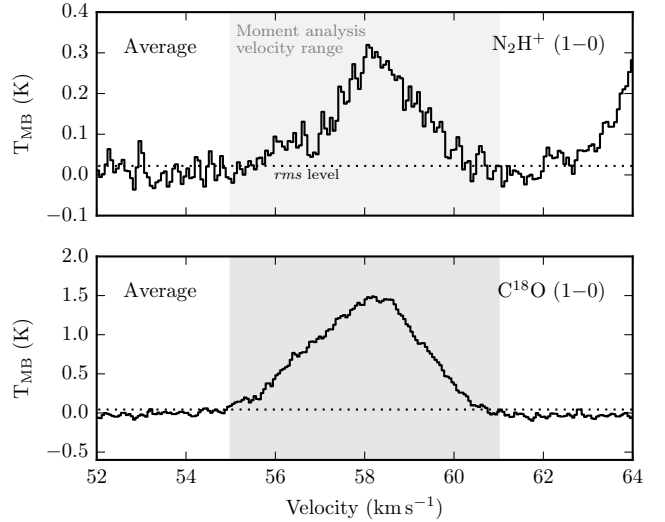
Figure 2. Shown are the average spectrum of the \text{N}_2\text{H}^+(1-0) transition (upper) and the \text{C}^{18}\text{O}(1-0) transition (lower) across the mapped region of Cloud F. The horizontal dotted line represents the rms level on the average spectrum of \sim 0.02 \text{ K} and \sim 0.04 \text{ K} for \text{N}_2\text{H}^+(1-0) and \text{C}^{18}\text{O}(1-0) , respectively. Note, these values are different to the average of the rms within individual positions, which is given in Table 2. The shaded region shows the velocity range used for the moment map analysis (see Figure 3).
