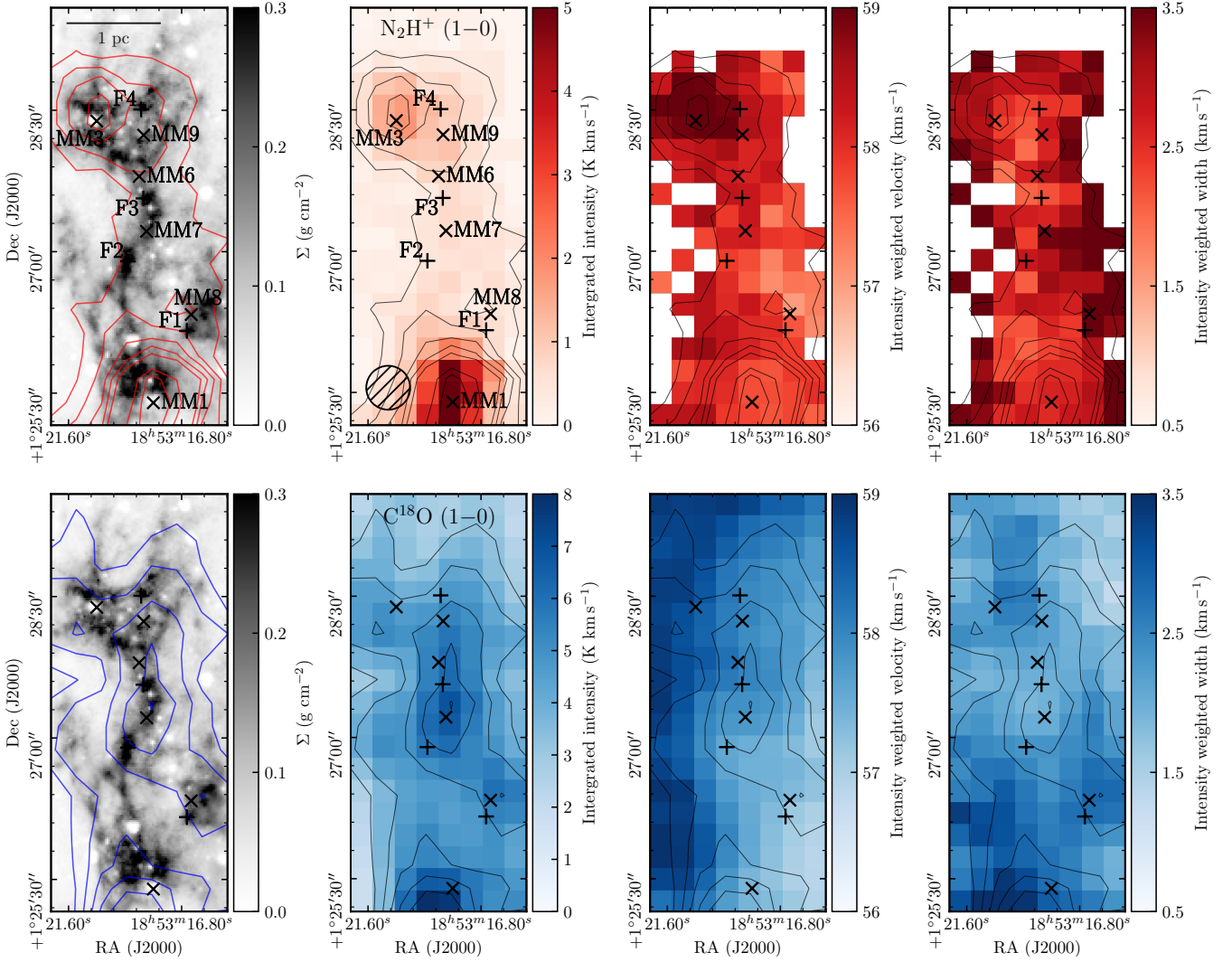
Figure 3. Moment map analysis of the Cloud F \text{N}_2\text{H}^+(1-0) (upper row) and \text{C}^{18}\text{O}(1-0) (lower row) observations. Shown in greyscale in the first column is the mass surface density map of Cloud F, determined from near- and mid-infrared extinction (Kainulainen & Tan 2013). Shown with + and x symbols are the positions of the “core” regions identified by Butler & Tan (2012) and those from Rathborne et al. (2006), respectively, which are labeled in both the upper left and upper centre-left panels. Shown in the second, third and fourth columns are the integrated intensities ( 0^{\text{th}} order moment), intensity weighted velocity field ( 1^{\text{st}} order moment), and intensity weighted line width ( 2^{\text{nd}} order moment) maps. Overlaid as red (first column) and black (second, third and fourth columns) contours in the upper row is the integrated intensity of \text{N}_2\text{H}^+(1-0) , in steps of \{5, 10, 15, 20, 25, 45, 55\} \sigma ; where \sigma \sim 0.08 \text{ K km s}^{-1} . Overlaid as blue (first column) and black (second, third and fourth columns) contours in the lower row is the integrated intensity of \text{C}^{18}\text{O}(1-0) , in steps of \{40, 50, 60, 70, 80\} \sigma ; where \sigma \sim 0.09 \text{ K km s}^{-1} . The moment analysis has been performed above 3\sigma for all transitions. Shown in the lower left corner of the second upper panel is the smoothed angular beam size.
