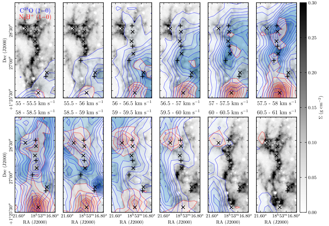
Figure 4. Cloud F channel maps of \text{N}_2\text{H}^+(1-0) and \text{C}^{18}\text{O}(1-0) shown in red and blue filled contours, which begin at 5\sigma , and increase in steps of 5\sigma , where \sigma \sim 0.023 \text{ K km s}^{-1} and \sigma \sim 0.024 \text{ K km s}^{-1} , respectively. The intensities are integrated from 55 - 61 \text{ km s}^{-1} in steps of 0.5 \text{ km s}^{-1} , as shown below or above each map. Each map is overlaid on the mass surface density map of Kainulainen & Tan (2013) . Shown with + and x symbols are the positions of the “core” regions identified by Butler & Tan (2012) and those from Rathborne et al. (2006) , respectively.
