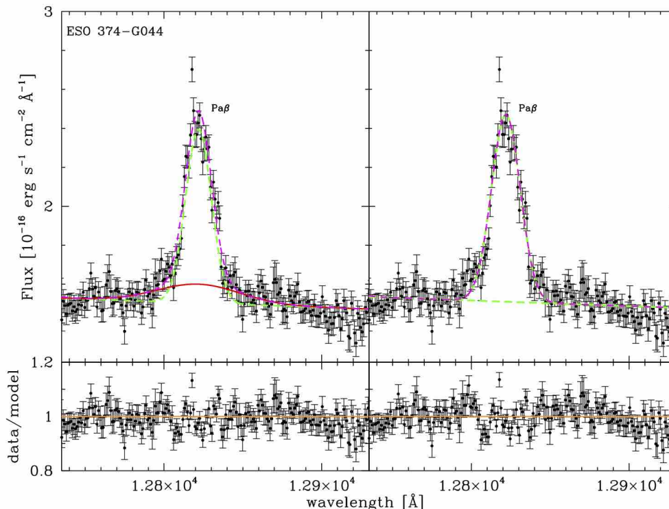
Figure A2. Left: Best fit of the Pa \beta lines of ESO 374–G044 including a broad (FWHM = 1413 km s −1 ) Pa \beta component. Right: Same as before without including the broad Pa \beta component. Lower panels show the data to model ratio.
