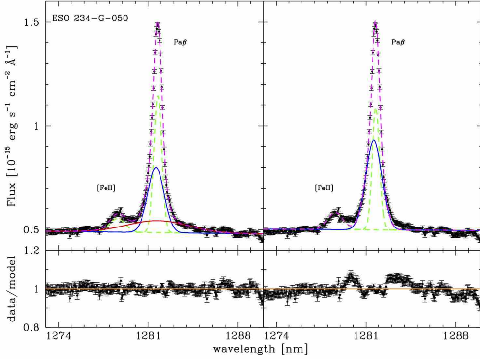
Figure A7. Left: Best fit of the \text{Pa}\beta line of ESO 234-G050 including a broad (FWHM = 1305 \text{ km s}^{-1} ) \text{Pa}\beta component. Right: Same as before without including the broad \text{Pa}\beta component. Lower panels show the data to model ratio.
