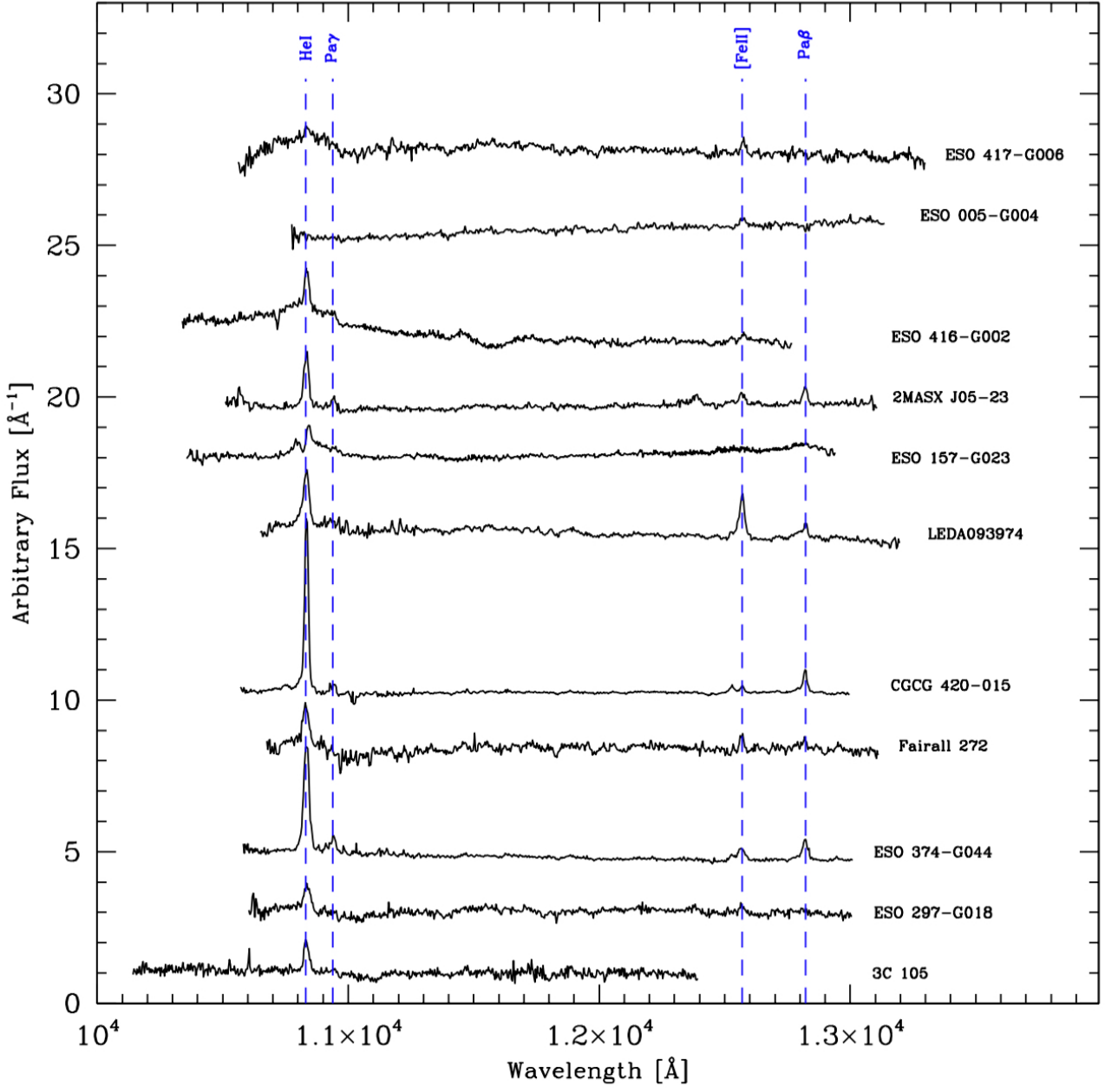
Figure 4. Low resolution NIR spectra, obtained with ISAAC/VLT, corrected for redshift. The rest frame wavelength position of some of the most relevant emission lines are shown by dashed vertical lines. The spectra are flux calibrated, but are shown with arbitrary normalization.
