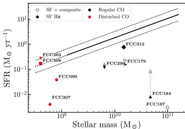
Figure 1. Location of the galaxies in the sample in the M_* - SFR plane (values are from Table 1), compared to the star formation main sequence (SFMS) from Elbaz et al. (2007) (solid line, the dashed lines represent the 1\sigma confidence interval, and the dotted line is an extrapolation towards lower masses). Filled markers indicate data points for which only the star-forming H \alpha was used and open markers indicate data points for which composite H \alpha was considered also. Both are plotted for each galaxy with the same marker shape, unless it contains only non-star-forming H \alpha (FCC167). Galaxies' FCC numbers are indicated. Galaxies with regular molecular gas reservoirs are shown in black and galaxies with disturbed molecular gas reservoirs in red (Section 2.1, Table 1). With few exceptions, galaxies in the sample lie below the SFMS.
