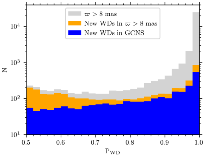
Fig. 36. Top: CAMD with the new WDs found here that were not included in Gentile Fusillo et al. (2019) , Torres et al. (2019) , or Jiménez-Esteban et al. (2018) . Bottom: probability distribution of the new WD candidates.
