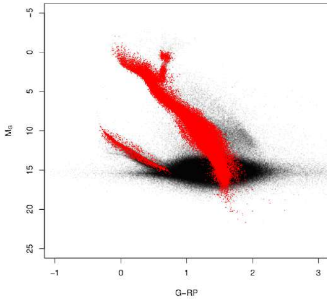
Fig. A.1. CAMD with colour G-R_{\text{P}} and absolute magnitude M_G of the set of sources with parallaxes greater than or equal to 8 mas (black) and those used as examples of good astrometry (red points) in the random forest training set.
