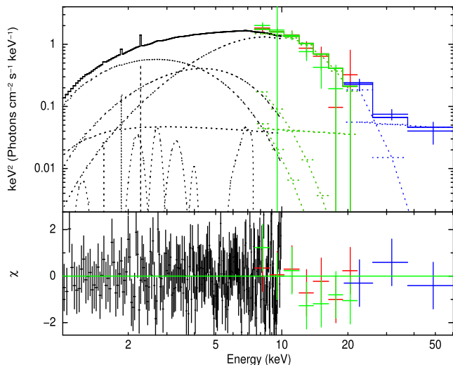
Figure 5. Unfolded E^2 f(E) XMM-Newton /EPIC-pn (black), INTEGRAL /JEMX-1 (red) and JEMX-2 (green) and INTEGRAL /ISGRI (blue). The dashed curves represent the best-fitting continuum (DISKBB, BB, NTHCOMP and POWER-LAW components) plus nine additional narrow and broad emission lines (see text).
