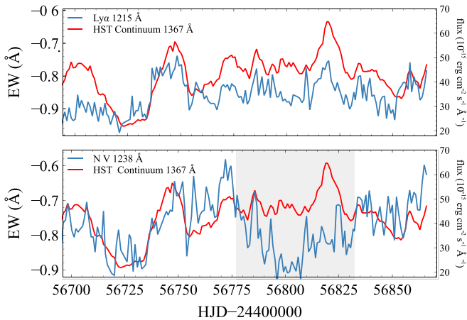
Figure 2. Both panels show the arbitrarily scaled FUV continuum in red, as a function of Heliocentric Julian Date -24,400,000 . The upper panel shows the equivalent width of the Ly \alpha absorber of Component 1 in blue and the lower panel shows the equivalent width of the corresponding N V \lambda 1238 absorption line. Shaded area indicates the time in which the “holiday” is happening.
