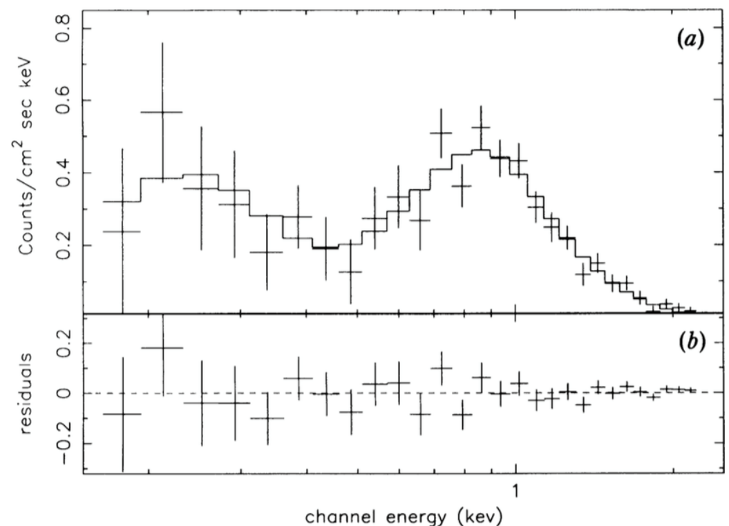
Figure 3. The ROSAT X-ray spectrum of the group NGC 2300 plotted together with the best-fit Raymond-Smith model (a) and residuals from the best fit model (b). Figure reproduced with permission from Reference [53].
