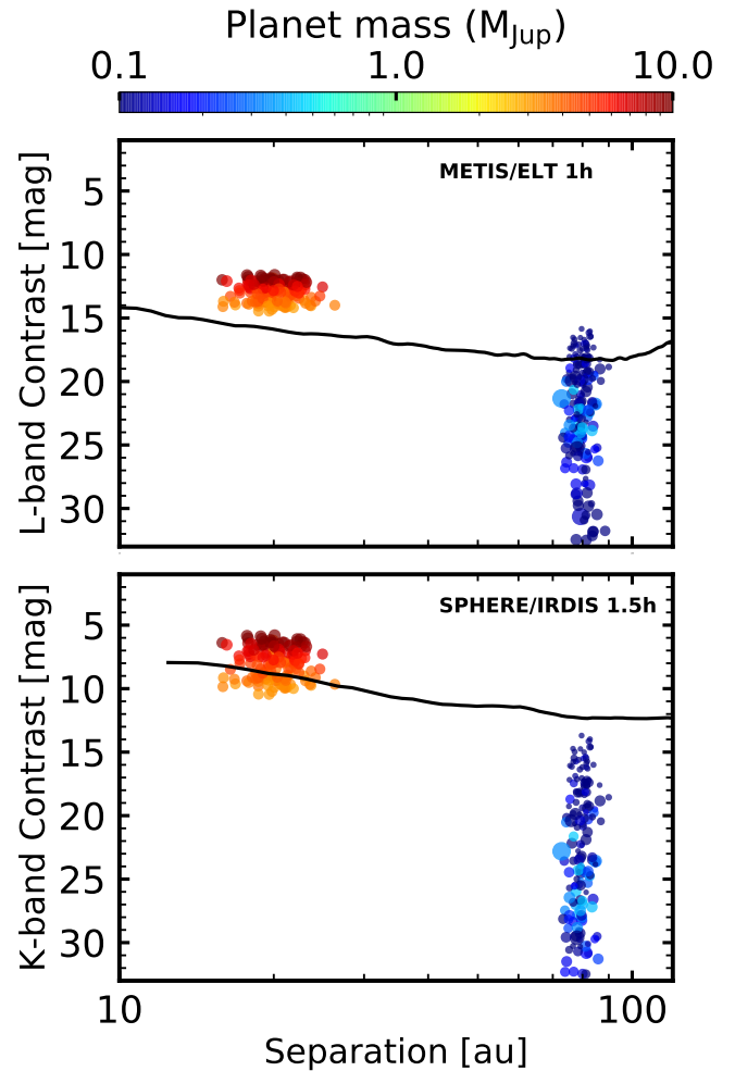
Fig. 11. Contrast magnitudes for 8 Myr planets in the NG76 population synthesis model (Emsenhuber et al. 2020, 2021). Two populations of 0.05\text{--}0.5 M_{\text{Jup}} and 3\text{--}10 M_{\text{Jup}} planets are artificially located at 80 and 20 au, respectively. Estimated extinction coefficients are from Sanchis et al. (2020) (see text). The METIS contrast curve is from Carlomagno et al. (2020), and the SPHERE limits correspond to the derived contrast in this work for RX J1604, which we adopt as a representative host star. Small random shifts in separation are applied for a better visibility of the populations, and dot sizes are connected to planet radius.
