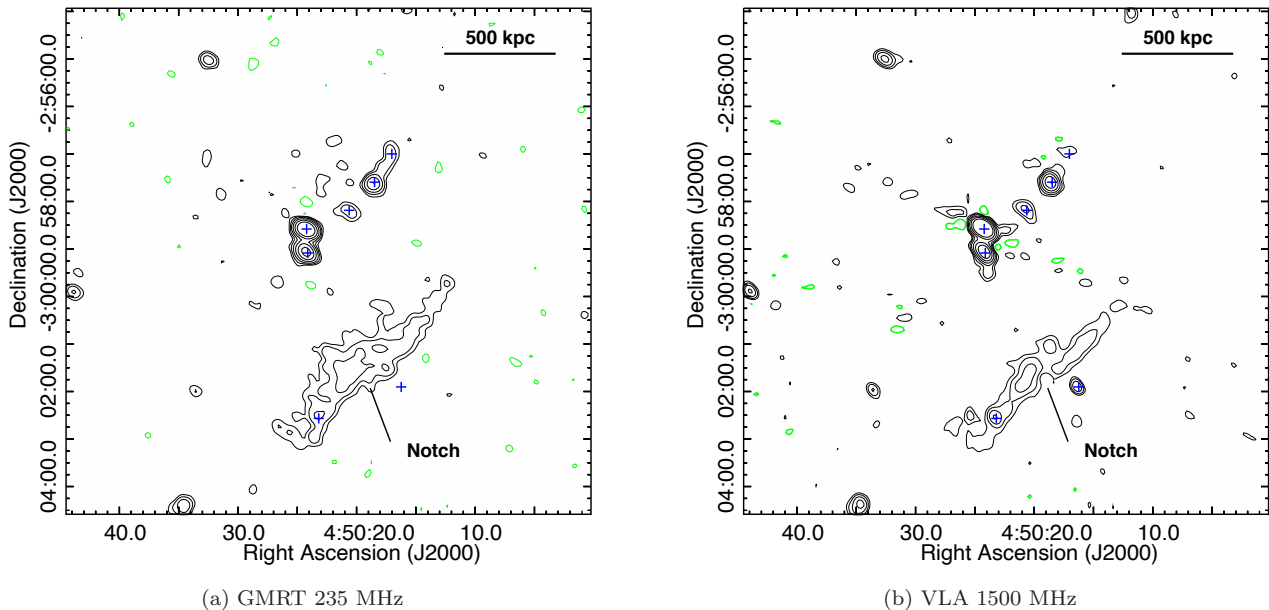
Figure 2. (a) – GMRT 235 MHz image with \sigma_{\text{rms}} = 0.39 mJy beam ^{-1} and resolution of 14.7'' \times 12.8'' , position angle 57.6^\circ is shown in contours. (b) – VLA 1.5 GHz image with a resolution of 14.5'' \times 10.0'' , position angle 33.7^\circ and \sigma_{\text{rms}} = 0.06 mJy beam ^{-1} is shown in contours. In panels a and b, the black are positive and the green are negative contour levels. The plus signs mark the discrete sources labelled in Fig. 1.
