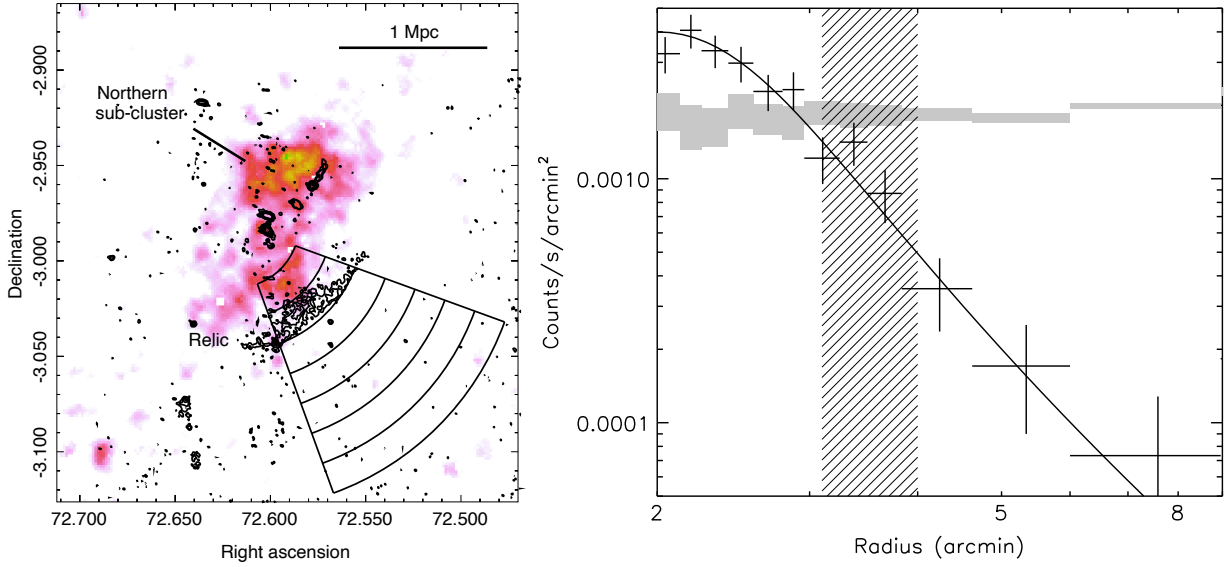
(a) XMM-Newton 0.4 - 1.4 keV with 610 MHz contours.
