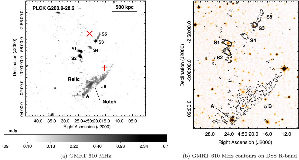
Figure 1. (a) – GMRT 610 MHz image is shown in grey scale. The 610 MHz image has a resolution of 5.6'' \times 4.7'' , position angle 59.4^\circ and rms noise, \sigma_{\text{rms}} = 0.045 mJy beam -1 . The discrete sources in the central region are labelled S1 – S5 and those near the extended source labelled ‘Relic’ are A and B. The symbols ‘×’ and ‘+’ mark the positions of the cluster according to the XMM-Newton and the Planck measurements, respectively. (b) – Digitized Sky Survey R-band image of the region of the labelled sources is shown in grey scale with the GMRT 610 MHz contours overlaid. The contour levels are 3\sigma_{\text{rms}} \times [\pm 1, 2, 4, \dots] mJy beam -1 .
