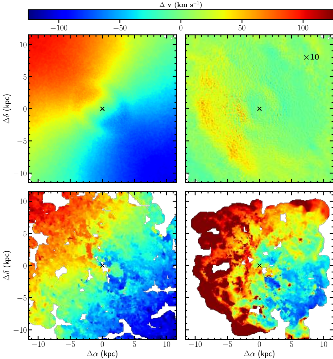
Fig. 22. Effects of the interaction on the kinematical properties of the perturbed galaxy. Upper left: stellar velocity map for the simulated unperturbed galaxy. Upper right: difference of the stellar velocity field of the perturbed vs. unperturbed model galaxy, with velocities multiplied by a factor of 10 for visibility. Lower left: velocity map of the molecular gas component for the simulated unperturbed galaxy. Lower right: velocity map of the molecular gas component for the simulated perturbed galaxy. All plots are for a simulated galaxy 50 Myr after the beginning of the interaction. The black cross shows the position of the photometric centre of the galaxy.
