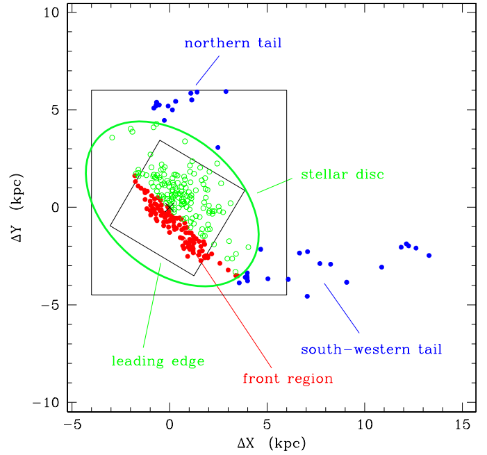
Fig. 4. Distribution of the HII regions of IC 3476 with luminosity L(H\alpha) \geq 10^{36} \text{ erg s}^{-1} and S/N > 5 . Filled red circles indicate HII regions in the front structure (101 objects), empty green circles indicate the other HII regions within the stellar disc (142), and filled blue symbols represent HII regions located outside the stellar disc of the galaxy (35), whose extension is measured within the r -band isophotal radius at 24 \text{ mag arcsec}^{-2} (from Cortese et al. 2012, see Table 1). The black cross shows the position of the photometric nucleus. The large black box shows the region of the Fabry-Perot data cube analysed in this work, while the small black box the field of view of MUSE IFU spectrograph, respectively.
