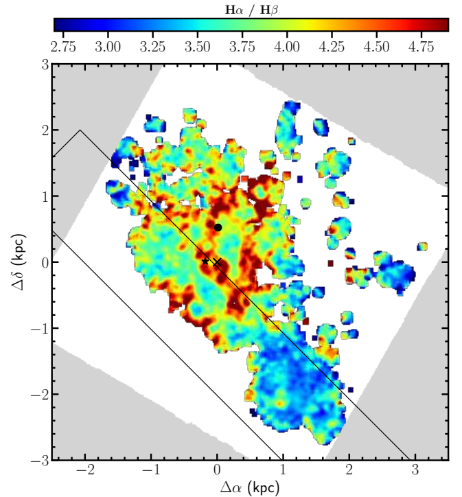
Fig. 8. Distribution of the Balmer decrement derived using the H\beta and H\alpha lines with an S/N > 5 . The black cross, star, and filled circle show the position of the photometric, stellar, and gas kinematical centres, respectively. The black rectangle indicates the front region of the galaxy (see Fig. 4).
