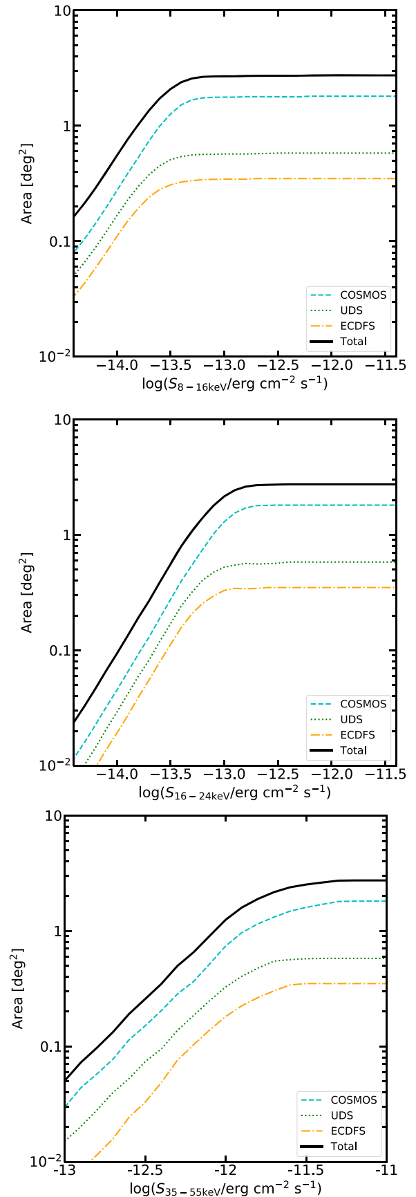
Figure 2. From top to bottom: sensitivity for the H1, H2, and H3 band, respectively. In each panel, the COSMOS curve is shown by the cyan dashed line, the UDS one in dotted green, and the ECFDS one in dotted-dashed orange. The total curve is the black thick line.
