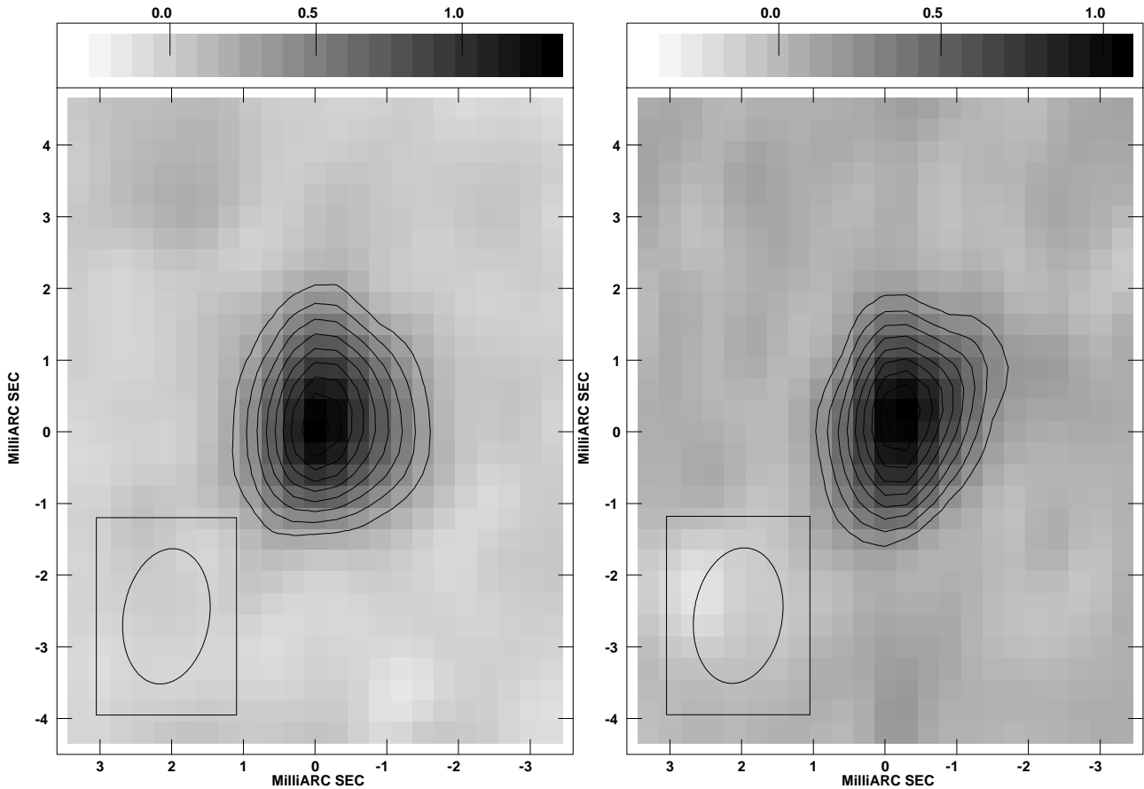
Fig. 3. VLBA maps of AR Lac at 8.4 GHz for Nov. 2–3 (left) and Nov. 3–4 (right). The rms of both maps is 0.06 mJy/beam and the peak intensity are 1.26 and 1.07 mJy, respectively. For the first map the contours correspond to 0.25, 0.38, 0.50, 0.63, 0.76, 0.88, 1.01, 1.13, 1.21 mJy, for the second map correspond to 0, 0.21, 0.32, 0.43, 0.54, 0.64, 0.75, 0.86, 0.96, 1.03 mJy. On the lower left corner the restoring beam is shown.
