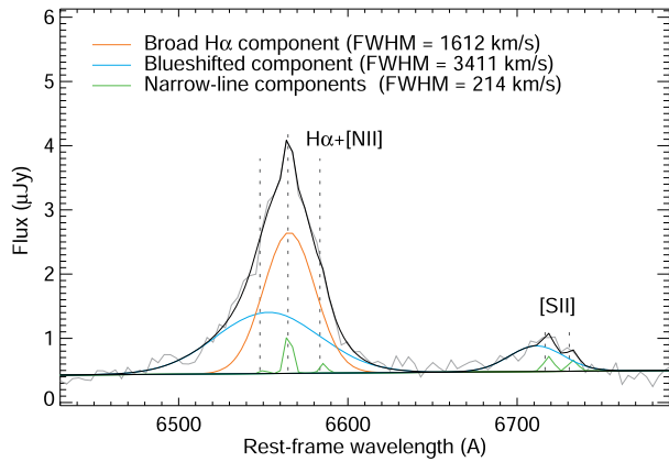
Extended Data Fig. 2 | H \alpha broad-line fitting. Left: The JWST NIRSpec spectrum (grey) with the best-fit model (black). The spectrum is extracted from a circular aperture of radius 0.2" centered on the central broad-line region. The power-law continuum (black), narrow-line components (green), broad-line components (orange), and outflow components (blue) are indicated. Dotted vertical lines
