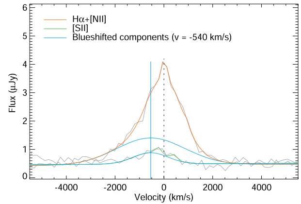
mark the line centers of the narrow-line components. Right: Comparison of the blue-shifted (outflow) line profiles of the H \alpha + [NII] and [SII] in velocity space. The blue-shifted (outflow) components are observed at a velocity of \sim -540 km/s relative to systemic.
