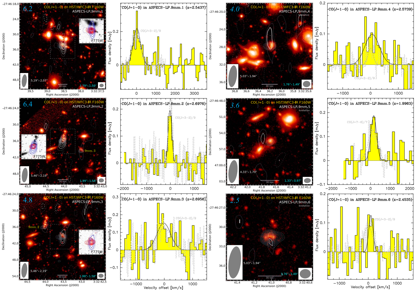
Figure 1. VLA CO( J = 1 \rightarrow 0 ) moment-0 line maps (left panels; white contours) and line spectra (right panels; solid histograms) of all detected galaxies in the sample, and Gaussian fits to the line profiles (black curves) where applicable. Contour maps are shown overlaid on HST/WFC3-IR F160W images, and ACS F775W insets for the robust detections (Illingworth et al. 2013), with CO( J = 1 \rightarrow 0 ) peak signal-to-noise ratios indicated in blue in the top left corner of each map panel. ALMA CO( J = 3 \rightarrow 2 ) or CO( J = 7 \rightarrow 6 ) (9mm.5 only) contours from González-López et al. (2019) or B20 are shown for comparison (aqua color). VLA maps are integrated over 737, 192, 923, 632, 405, and 341 \text{km s}^{-1} (80, 20, 96, 68, 52, and 38 MHz), for 9mm.1, 2, 3, 4, 5, and 6, respectively. VLA contour levels are in steps of 1\sigma = 14, 25, 12.5, 14, 30, and 20.2 \mu\text{Jy beam}^{-1} , starting at \pm 2\sigma (except 9mm.6, where an additional 2.5\sigma contour level is shown). ALMA contour levels are in steps of 1\sigma = 27, 65, 38, 37, 105, and 29 \mu\text{Jy beam}^{-1} , starting at \pm 3\sigma , except 9mm.1, where contour steps are \pm 3\sigma . The VLA (ALMA) beam sizes are shown in the bottom left (right) corner of each panel. 9mm.5 shows an offset between the peak position of both lines, likely primarily due to the modest signal-to-noise ratio of the tentative CO( J = 1 \rightarrow 0 ) detection. Spectra are shown at resolutions of 74, 77, 77, 74, 149, and 72 \text{km s}^{-1} (8, 8, 8, 8, 16, and 8 MHz), respectively. Velocity scales are relative to the redshifts indicated. Scaled ALMA CO( J = 3 \rightarrow 2 ) or CO( J = 7 \rightarrow 6 ) spectra (dashed gray histograms; González-López et al. 2019; B20) are shown for comparison.
