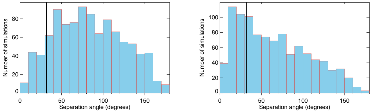
Fig. 10. Angular distance between hot or cold spot and direction of max dipolar modulation. The distribution of the angular distance is shown for 1000 Gaussian simulations (left panel) and 1000 non-Gaussian simulations (right panel). The vertical black line corresponds to the angular distance for the Planck data.
