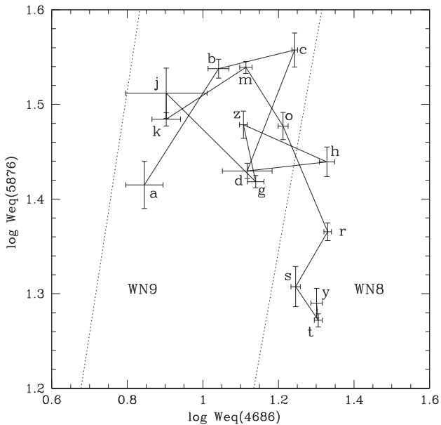
Figure 5. Time evolution of the equivalent width of He II 4686 Å and He I 5876 Å to mark the path of GR 290 through the WN sub-classes during its luminosity variations from 2005 August to 2015 December. The letters correspond to the following dates: a = 2005 August 31; b = 2005 November 08; c = 2006 December 14; d = 2007 January 29; h = 2008 February 07; z = 2008 September 08; g = 2010 January 21; j = 2010 December 18; k = 2011 August 03; m = 2011 September 20; o = 2012 December 09; r = 2013 November 27; s = 2014 January 01; t = 2014 December 11; y = 2015 December 11.
