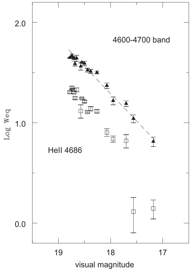
Figure 6. Logarithm of the equivalent width of the He II 4686 Å line (open squares) and the 4600–4700 Å emission feature (triangles) vs. visual luminosity during 2003 January–2015 December. The fit of the data points described in the text is shown.
