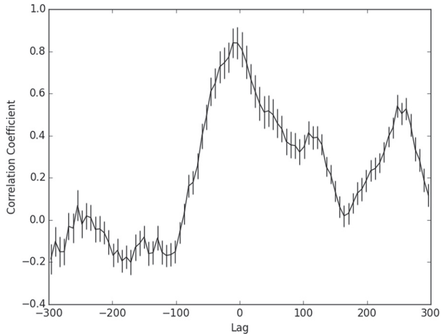
Figure 6. Discrete cross-correlation function (seven-day bin) between 100 MeV–300 GeV and R -band data.
