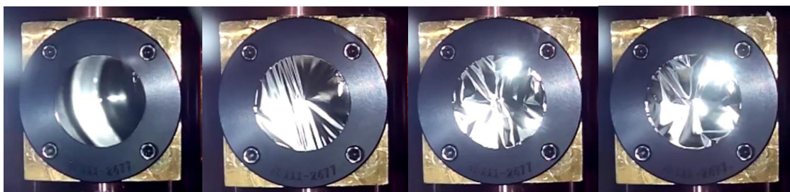
Figure 2. Test filter TF111-2677 in UHV ( P = 2.5 \cdot 10^{-9}\text{ mbar} ) at 300 K, 250 K, 220 K, 158 K from left to right. Pictures are taken from a side view port of the vacuum chamber.
