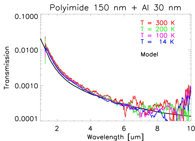
Figure 5. IR Transmission measurements performed on sample TF111-2677 (Polyimide 150 nm/Al 30 nm) at 4 different temperatures in the range 14-300 K. Superimposed is also the modeled transmission (black solid line).
