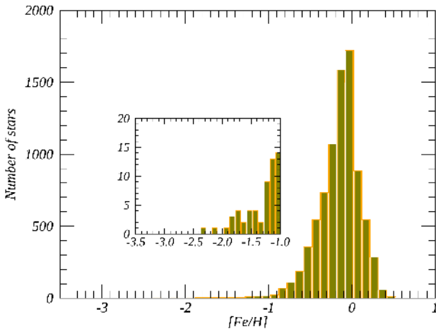
Fig. 8. Histogram of [\text{Fe}/\text{H}] for the sample of field stars. In the inset we show the tail at low [\text{Fe}/\text{H}] .
