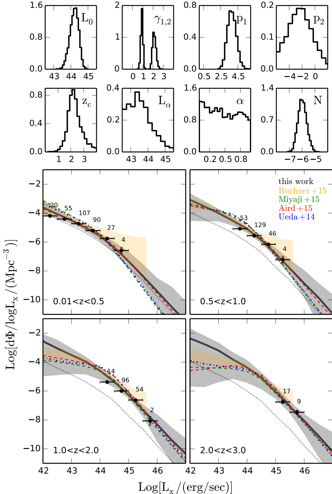
Fig. 10. X-ray luminosity function from the XXL-1000-AGN sample. The upper panels show the marginalized posterior distribution of the parameters in luminosity dependent density evolution (LDDE) model. The bottom panels show the estimated XLF as a function of luminosity in four redshift bins. The black solid line shows the mode of the distribution and the grey shaded area encloses the 90% credible interval. The dotted black line is our estimated z = 0 XLF shown for reference in all plots. The black points are estimated using the 1/V_{\text{max}} method in good agreement with our modelling. The numbers above the points show the number of objects per bin. They also show the parameter space occupied by the XXL-1000-AGN sample. The orange area and dashed lines show 2–10 keV XLF estimates from the literature (orange: Buchner et al. 2015; green: Miyaji et al. 2015; red: Aird et al. 2015; blue: Ueda et al. 2014).
