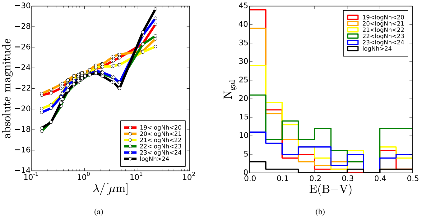
Fig. 7. a) Median rest-frame SEDs for X-ray counterparts from UV to mid-infrared for XXL-N sources and b) Values of optical absorption E(B-V) estimated from the broadband SEDs and split into N_{\text{H}} bins determined from the X-ray spectrum, ranging from unabsorbed (red) to Compton-thick sources (black).
