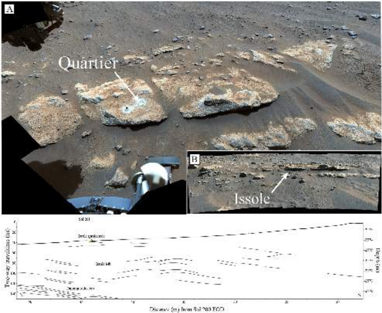
Figure 4. Mastcam-Z workspace mosaics and interpreted RIMFAX subsurface for Issole: The Séítah formation outcrop target near the Séítah/Máaz contact. (a) Sample borehole (~1.3 cm diameter) and Quartier abrasion site (~5 cm diameter) in workspace image provide scale of targeted outcrop features. (b) View of Issole looking south from Séítah towards base of the Artuby Ridge (not seen).
