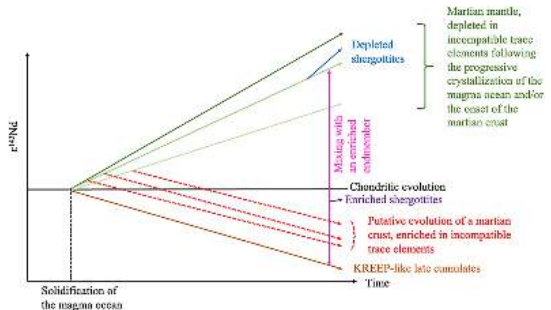
Figure 16. Schematic geodynamical evolution of the martian interior : Radiogenic ingrowth of ^{143}\text{Nd}/^{144}\text{Nd} depends on the variation in Sm/Nd in the reservoirs. The progressive solidification of the magma ocean resulted in several depleted reservoirs (in green) and ended up with enriched late cumulates (in brown), after Debaille et al. (2007). From the depleted martian mantle, a crust has been extracted, that is enriched in incompatible trace elements, as observed in NWA 7034 (Armytage et al., 2018). Depleted shergottites (in blue) directly sample a depleted reservoir while the enriched shergottites (in violet) represent a mixture (in pink) between depleted and enriched reservoirs.
