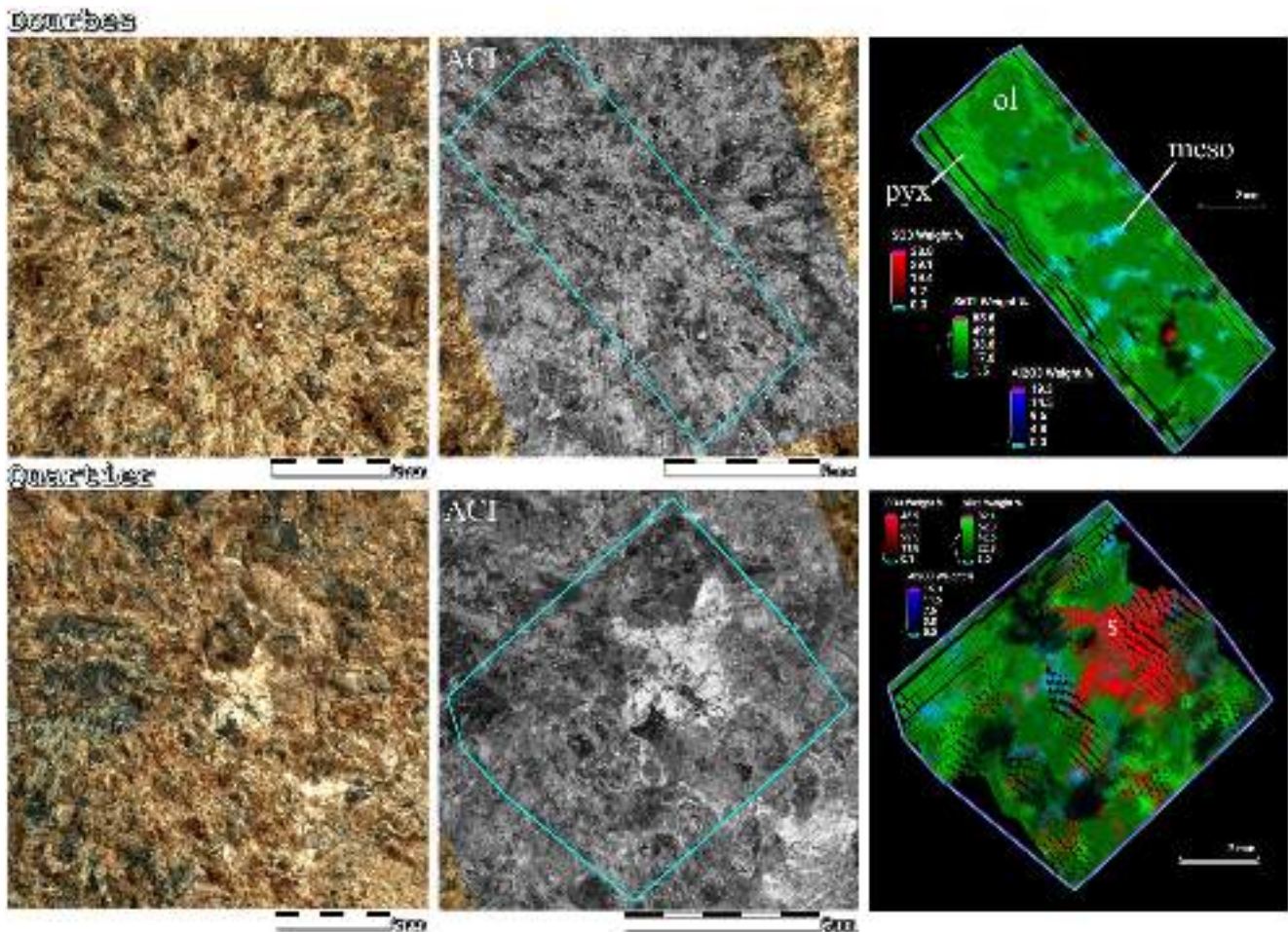
Figure 9. Close up observations of Séítah abrasion sites by WATSON (~4 cm standoff), Autofocus and Context imager, and PIXL: Compositional X-ray map of SO 3 (red), SiO 2 (green), and Al 2 O 3 (blue) concentrations, generally correspond to primary olivine (ol) = dark green and pyroxene (pyx) = light green, compositionally evolved intercumulus mesostasis (meso) = blue and secondary sulfate (s) = red, respectively (see text and Figures S12–S16, Table S1 in Supporting Information S1 for additional information).
