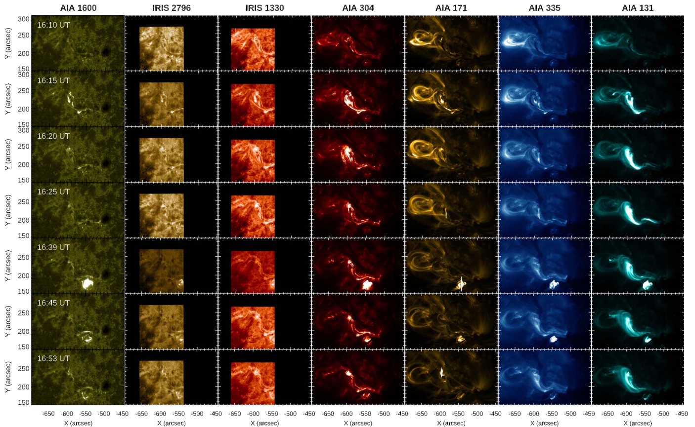
Figure 4. Synoptic view of the evolution of the C7.0 flare at different atmospheric layers, at representative times during the observing interval. From left to right, each row shows the SDO/AIA 1600 Å map, the IRIS SJI 2796 Å and 1330 Å maps, and the SDO/AIA cospatial maps for the selected EUV channels.
