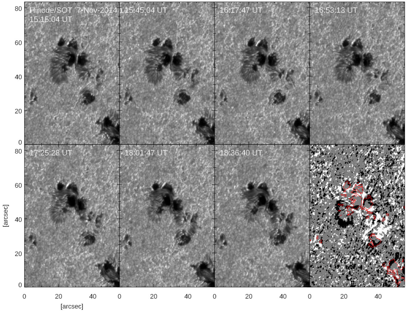
Figure 12. Panels 1–7: photospheric evolution of \delta -complex A during the C7.0 and X1.6 flares, as seen by Hinode /SOT in G band. Bottom-right panel: difference image between the first and last G-band filtergrams of the Hinode /SOT sequence. White (black) areas indicate regions with penumbral enhancement (decay). Red contours indicate the umbral boundary at the beginning of the sequence.
