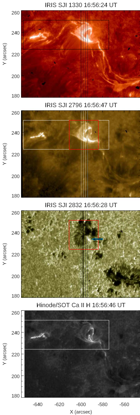
Figure 5. Top panels: maps derived from IRIS SJI images acquired on 2014 November 7 at around 16:56 UT, showing a portion of the FOV recorded by the instrument at three different wavelengths: SJI 1330 Å (first panel), SJI 2796 Å (second panel), and SJI 2832 Å (third panel). In each image, the dashed vertical lines indicate the raster positions during the acquisition time. Bottom panel: Hinode / SOT Ca II H filtergram simultaneous with IRIS SJI images. The solid-line box indicates the sub-FOV analyzed in Figure 6. The red-line box frames the sub-FOV zoomed in Figure 7. The arrow in the third panel indicates the brightening. An animation of the Hinode / SOT Ca II H images is available. The video begins at 16:51:47 UT and ends on 17:05:47 UT. The real-time duration is 5 s. The ejection of the flux rope is clearly visible.
