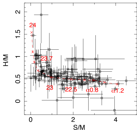
Fig. 10: Colour-colour (H/M - S/M) diagram for the midz and highz sources. The locus in dashed red line indicates the evolution of (S/M, H/M) when a power-law continuum of energy index \alpha = 0.8 is modified by cold absorption with various column densities: \log N_H [cm ^{-2} ] of 22, 22.5, 23, 23.5, 23.7, 23.85 and 24, as marked by cross symbols. Colours for a simple power-law with no absorption with \alpha of 0.8, 1.0, and 1.2 are also marked.
