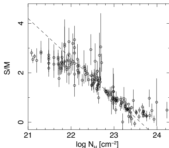
Fig. 9: Plot of S/M colours against best-fitting N_H , obtained from the conventional spectral fit. The dashed line indicates the best-fitting relation in the range of 22-23.3 in \log N_H [cm ^{-2} ] (see text).
