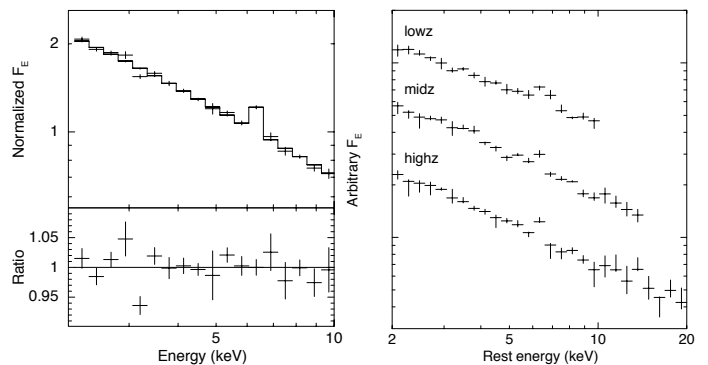
Fig. 15: Left panel: Composite spectrum of all the 81 unobscured AGN with the best-fit power-law plus a narrow Gaussian for the Fe K emission and the residual in ratio of the data and the model. Right panel: Composite spectra of unobscured sources in the lowz, midz and highz groups. The spectra are plotted with arbitrary offsets for clarity.
