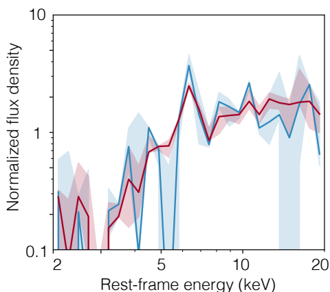
Fig. 19: Composite spectra of the seven Compton-thick AGN candidates selected by spectral fitting (blue) and 19 candidates filtered by the two X-ray colours, S/M and H/M , and R(\text{Fe}) alone (red).
