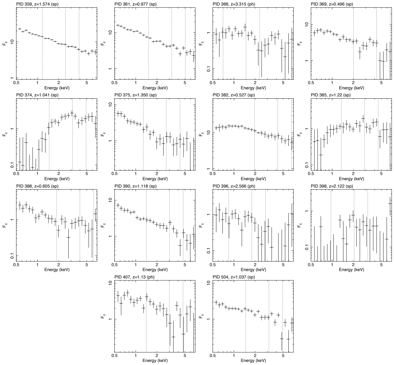
Fig. D.1: Observed 0.5-7 keV spectra of the remaining 182 XMM-CDFS sources of Fig. 2. Flux density is in units of 10^{-15} \text{erg s}^{-1} \text{cm}^{-2} \text{keV}^{-1} . The energy scale is as observed and the three, vertical dotted lines indicate the rest-frame energies of 3 keV, 6.4 keV and 10 keV, expected from the adopted redshift.
