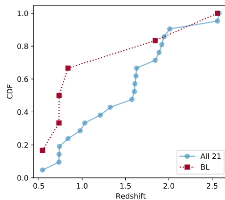
Fig. 8: Cumulative distribution functions of the redshifts of the 21 unobscured AGN with good data quality (blue circles) and those of the six in which broad Fe lines are detected (red squares). The redshifts of the sample AGN are spread over the range of 0.5-2.6 with some clustering in the z = 1.6-2 range. In contrast, broad line detections may be frequent at low redshifts ( z < 0.9 ).
