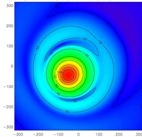
Figure 8 Feed horn 18: contour plot projection on SKL surface. The most power (>0.99) is located in a region with diameter d < 150\text{mm} . Other feeds have similar behaviours or, at least, comparable.
