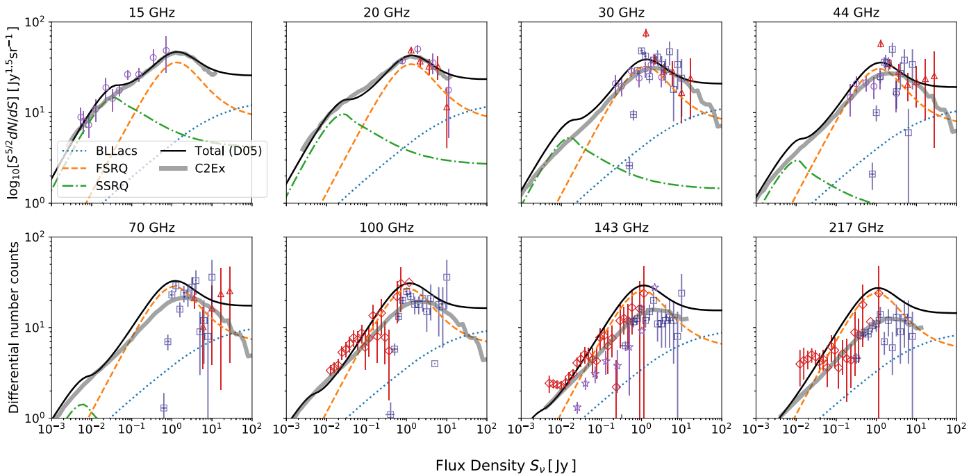
Figure 6. Euclidean normalized differential number counts on a wide range of frequencies. The dotted, dashed, dotted–dashed and solid lines are respectively the number counts of BL Lacs, FSRQs, SSRQs and their total contribution predicted by the D05 model. The thick solid gray line are the number counts coming from the C2Ex model. Number counts obtained with several experiments observing at similar frequency channels are also shown: open circles at 15 and 20 GHz are, respectively, from Waldram et al. (2003, 2010) and Massardi et al. (2008); open circles at 30 and 44 GHz resemble counts from the PACO data set (Bonavera et al. 2011); upper triangles from 20 to 70 GHz are data from WMAP5-yr survey (Massardi et al. 2009); diamonds at 100, 143, and 217 GHz are from SPT (Mocanu et al. 2013); stars at 143 GHz are ACT counts (Marriage et al. 2011); squares at 30, 44, 70, 100, 143, and 217 GHz are based on data from Planck Collaboration et al. (2011b).
