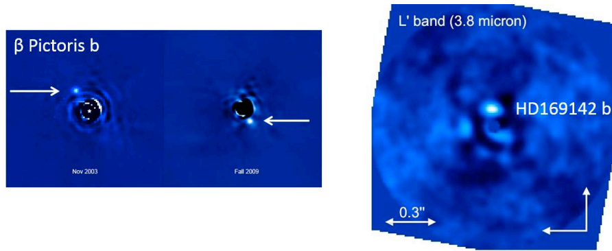
Figure 3. Key L-band detections of exoplanets made by NACO. Left: \beta Pictoris b is a 4–11 M_{Jup} planet orbiting at a distance of 9 AU from the star in a plane close to that of the debris disk at larger scales. 15,16 Right: HD169142 b is a protoplanet that has not been observed at shorter wavelengths, located in the transition disk around the star. 17,18 SAMs and coronagraphs, in combination with Angular Differential Imaging (ADI), significantly ease the detection of such objects.
