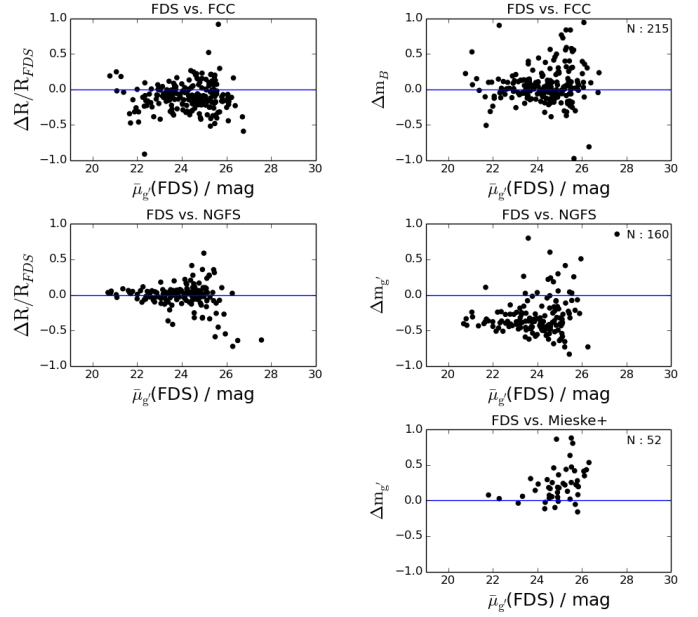
Fig. 24. Effective radii ( R_e , left panels) and apparent magnitudes ( m_B/g' , right panels) of the galaxies obtained in this work are compared to those given in FCC, NGFS (Eigenthaler et al. 2018), and Mieske et al. (2007), from the top to bottom rows, respectively, using the galaxies common in the studies. The differences are with respect to FDS values, i.e., \Delta X = X_{\text{FDS}} - X_{\text{Ref.}} . The x -axis shows the mean effective surface brightness ( \bar{\mu}_{e,g'} ) of the galaxies, and the blue lines show the zero off-sets. Mieske et al. (2007) does not include effective radii for the galaxies, and therefore the comparison is not shown. The number of galaxies in common between the studies are marked into the upper right corners of the right-side panels.
