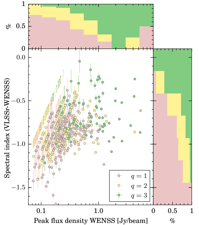
Fig. 7. Source quality as a function of low-frequency spectral index and WENSS peak flux density. Red, yellow, and green colours represent q = 1, 2 , and 3 , respectively. q = 3 corresponds to suitable primary calibrators. The histograms show the percentage of sources at each quality value. The histogram on the right does not include the sources with upper limits in their spectral indexes. The uncertainties of some of the values are smaller than the symbols, especially for the WENSS peak flux density. The stripes at low peak flux densities are due to sources detected at multiples of the rms noise of VLSSr.
