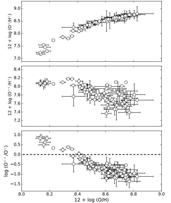
Figure 7. The \text{O}^+ abundance (upper panel), the \text{O}^{++} abundance (middle panel) and the relative ionic abundance of the two species (bottom panel) are shown as a function of the total oxygen abundance.
