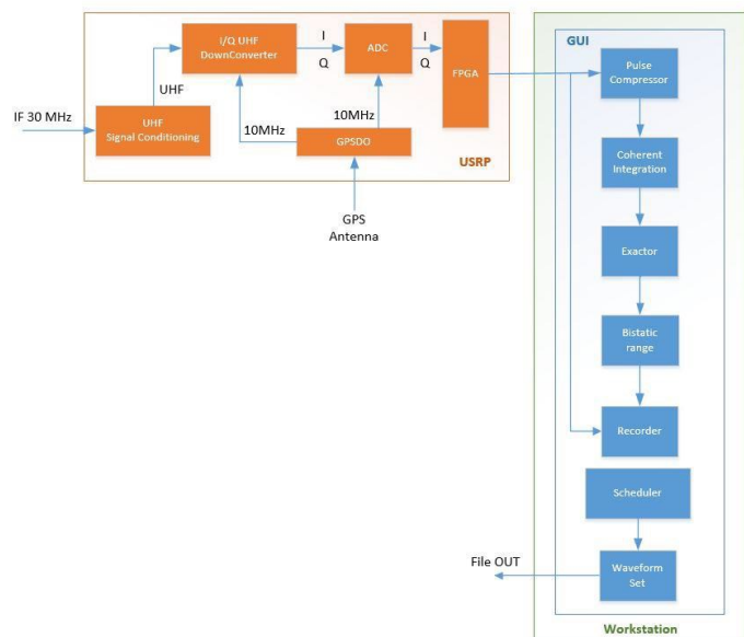
Fig. 4. The receiver architecture.
