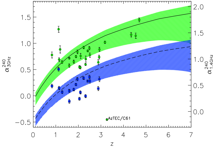
Fig. 2. Modeled radio-mm spectral indices, \alpha as a function of redshift. The solid and dashed lines correspond to \alpha_{3\text{ GHz}}^{240} and \alpha_{1.4\text{ GHz}}^{240} , respectively, while the green and blue hashed regions correspond to the uncertainty range due to varying dust SED temperatures spanning 25 to 60 K. The axes for the two spectral indices have been offset for clarity. Green circles and blue squares indicate those sources in our sample with spectroscopic redshifts which are detected at 3 and 1.4 GHz, respectively. AzTEC/C61 demonstrates an inverted radio spectrum and is suspected of hosting an AGN, so its extreme spectral index is not used as a redshift indicator (Miettinen et al. 2017a).
