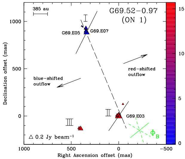
Fig. 6. View of the CH 3 OH maser features detected around G69.52-0.97 (Table A.4). Same symbols as in Fig. 1. The polarization fraction is in the range P_l = 1.3-1.5\% (Table A.5). The assumed velocity of the YSO is V_{\text{lsr}}^{\text{CS}} = +11.6 \text{ km s}^{-1} (Bronfman et al. 1996). The dashed line is the best least-squares linear fit of the CH 3 OH maser features ( \text{PA}_{\text{CH}_3\text{OH}} = +23^\circ \pm 7^\circ ). The two arrows indicate the direction and not the actual position of the red- and blueshifted lobes of the outflow ( \text{PA}_{\text{outflow}}^{\text{CO}} = -69^\circ , Kumar et al. 2004).
