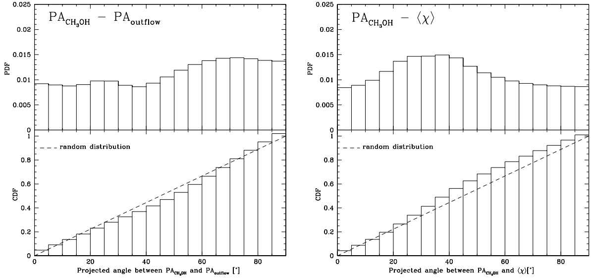
Fig. 8. Probability density function and CDF of the projected angle between the PA of the CH 3 OH maser distribution and the outflow axis ( |\text{PA}_{\text{CH}_3\text{OH}} - \text{PA}_{\text{outflow}}| ) (left). Right: Probability distribution function (top panel) and CDF (bottom panel) of the projected angle between the PA of the CH 3 OH maser distribution and the linear polarization angles ( |\text{PA}_{\text{CH}_3\text{OH}} - \langle\chi\rangle| ). In both panels the dashed line is the CDF for random distribution of the corresponding angles, i.e., all angular differences are equally likely. The results of the K–S test are listed in Table 3.
