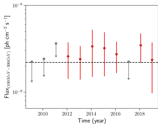
Fig. 3. Fermi -LAT one-year binned light curve of NGC 3894. The dashed line represents the averaged flux for the entire period Flux_{10.8\text{ years}} = 2.2 \times 10^{-9} \text{ ph cm}^{-2} \text{ s}^{-1} .
