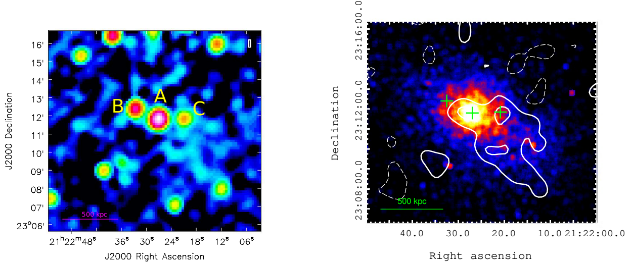
Fig. 5. JVLA image of the cluster Z2120. Left: JVLA D array image. The resolution is 33'' \times 30'' and the rms noise is 0.06 mJy beam -1 . Labels mark the discrete sources in the cluster field. Right: low-resolution ( 55'' \times 54'' ) JVLA contours after the compact sources subtraction overlaid over the X-ray Chandra image. Contours are drawn at (3, 6, \dots) \times \sigma , with \sigma = 0.1 mJy beam -1 . The 2\text{-}\sigma negative contour is dashed. The green crosses mark the position of the three sources at the cluster centre, which have been subtracted.
