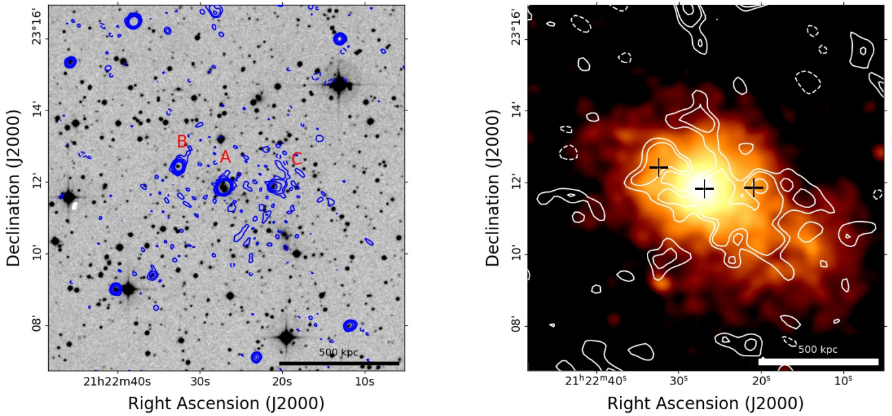
Fig. 6. GMRT images of the cluster Z2120. Left: DSS optical image with GMRT high-resolution contours overlaid. Contours start at 0.1 mJy beam -1 and are spaced by a factor of two. The first negative contour is dashed. Labels mark the position of discrete sources. Right: GMRT 330 MHz low-resolution ( 32.7'' \times 28'' ) contours after the subtraction of compact sources superimposed on the Chandra X-ray image. Contours are (2, 3, 6, \dots) \times \sigma , with \sigma = 0.3 mJy beam -1 . The position of the discrete sources is marked with a black cross.
