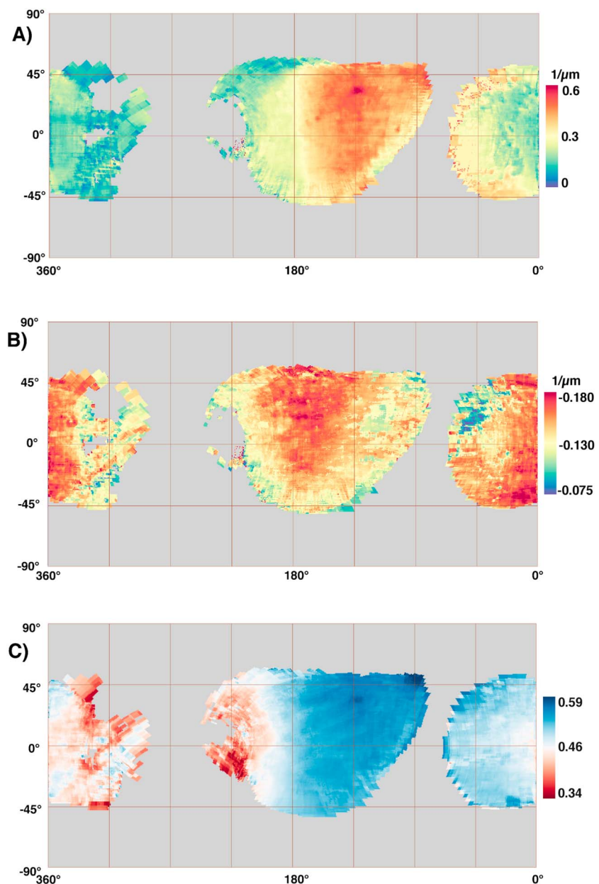
Figure 4. Dione cylindrical maps for 0.35–0.55 μm slope (a), 0.55–0.95 μm slope (b), and 2.050 μm water ice band depth (c).
