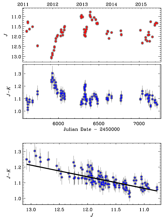
Figure 3. The J -band light curve in the 2011–2015 period (top panel); the corresponding J-K colour index as a function of time (middle panel) and brightness level (bottom panel). In the bottom panel the solid line represents a linear fit to the data. The data have been corrected for the host galaxy contribution.
