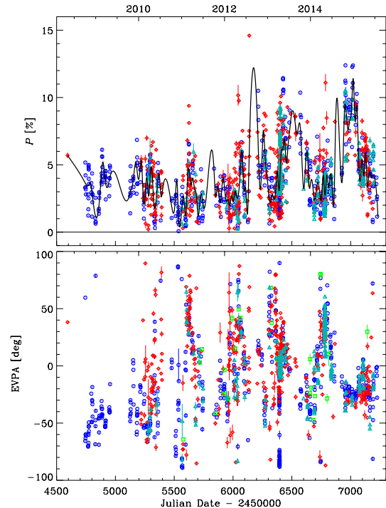
Figure 14. Top: the observed degree of polarisation as a function of time; the black line represents a cubic spline interpolation through the 15-d binned data. Bottom: the observed EVPAs in the -90^\circ and +90^\circ range. Data are from the Calar Alto (green squares), Crimean (red diamonds), Lowell (cyan triangles) and Steward (blue circles) observatories.
