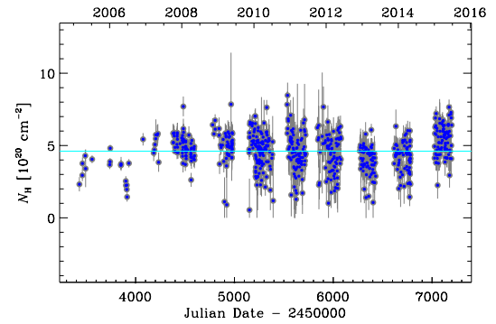
Figure 9. The Galactic Hydrogen column N_{\text{H}} as a function of time when a power-law model with free absorption is applied to the XRT spectra. The cyan line marks the average value.
