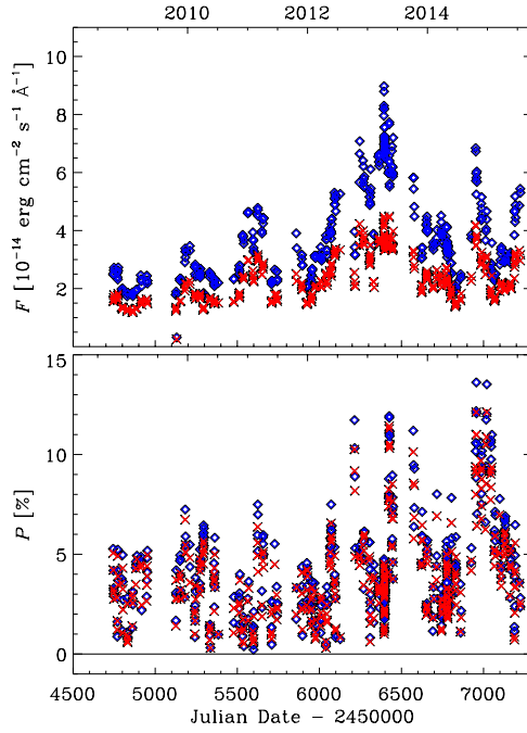
Figure 23. The observed optical flux density (top) and polarisation percentage (bottom) as a function of time in the blue and red bins defined in the text.
