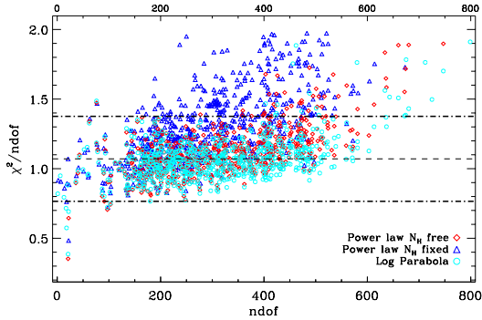
Figure 6. Reduced \chi^2 versus the number of degrees of freedom for the different models applied to the XRT spectra of Mrk 421. Blue triangles represent the results of the power-law model with N_{\text{H}} fixed to the Galactic value, red diamonds those of the power-law model with N_{\text{H}} free, and the cyan circles those of the log-parabola model with Galactic N_{\text{H}} .
