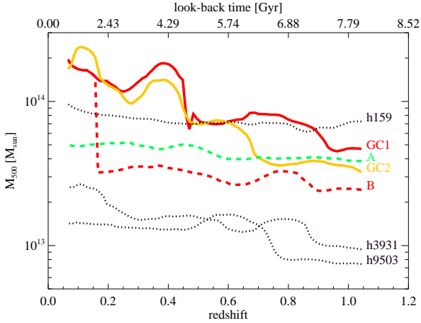
Fig. 13. Redshift evolution of the total mass M_{500} for all the clusters and groups identified at z=0.07 in the (20 h^{-1} \text{cMpc})^3 volume around the cluster pair. At each redshift up to z \sim 1 , we consider the main progenitor of the given halo identified at z=0.07 .
