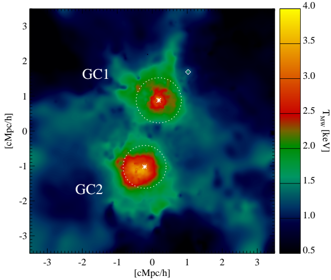
Fig. 7. Projected mass-weighted temperature map of the galaxy cluster pair at z=0.07 . The map is centred on the system centre of mass and is 7 h^{-1} cMpc per side, and the integration along the l.o.s. is also performed over 7 h^{-1} cMpc. The dotted white circles indicate the R_{500} radii of GC1 and GC2. The position of group B (diamond) is also marked.
