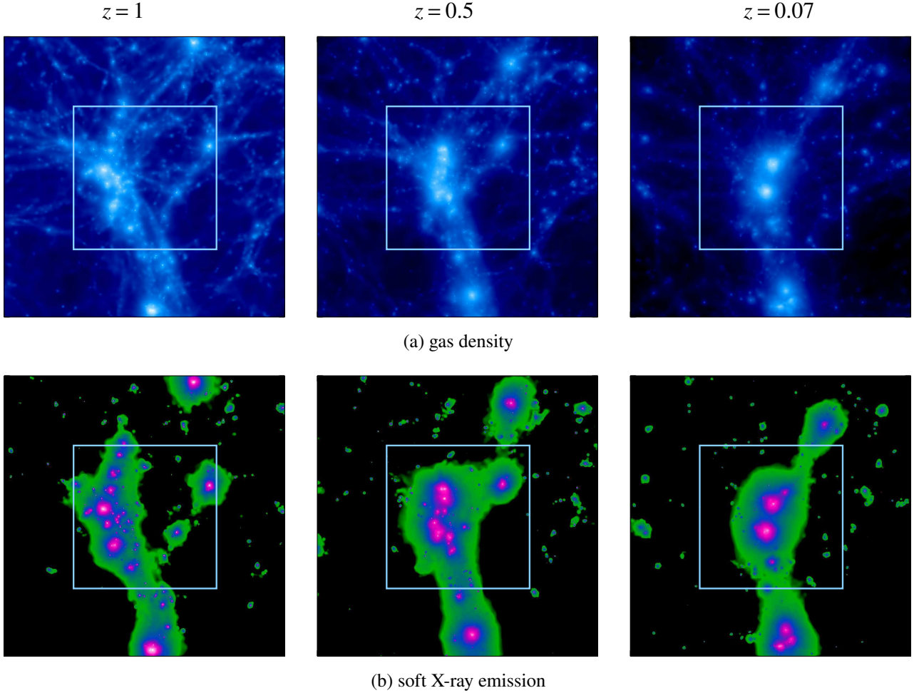
Fig. 2. Projected maps of gas density and ideal X-ray emission in the [0.5–2] keV band. Each map is 20 h^{-1} cMpc per side, integrated for 20 h^{-1} cMpc along the l.o.s. ( z -axis) and centred on the pair centre of mass at z = 0.07 . The squares ( 10 h^{-1} cMpc per side) approximate the size of the eROSITA observation.
