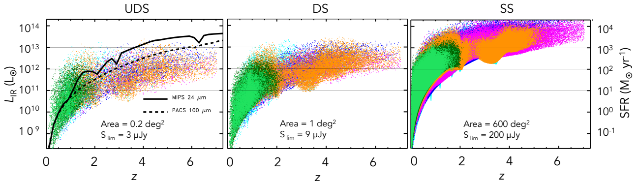
Figure 7. Expected total IR luminosity (SFR) as a function of redshift for the three photometric surveys planned with SPICA-SMI/CAM ( left : UDS to 3 \mu\text{Jy} ; middle : DS to 9 \mu\text{Jy} ; right : SS to 0.2 \text{ mJy} ). The different colours of the points represent the behaviour of different SED-types: cyan, starburst ; green, spiral ; dark-green, SF-AGN(spiral) ; orange, SF-AGN(SB) ; magenta, AGN2 ; and blue, AGN1 (see Gruppioni et al. 2013 for details and the text for a brief description of these populations). For comparison, the limiting IR luminosity corresponding to the fluxes reached by the deepest surveys with Spitzer (MIPS 24 \mu\text{m} ) and Herschel (PACS 100 \mu\text{m} ) are shown in the left panel as black solid and dashed lines respectively. The horizontal lines mark the LIRG, ULIRG and HyLIRG limits.
